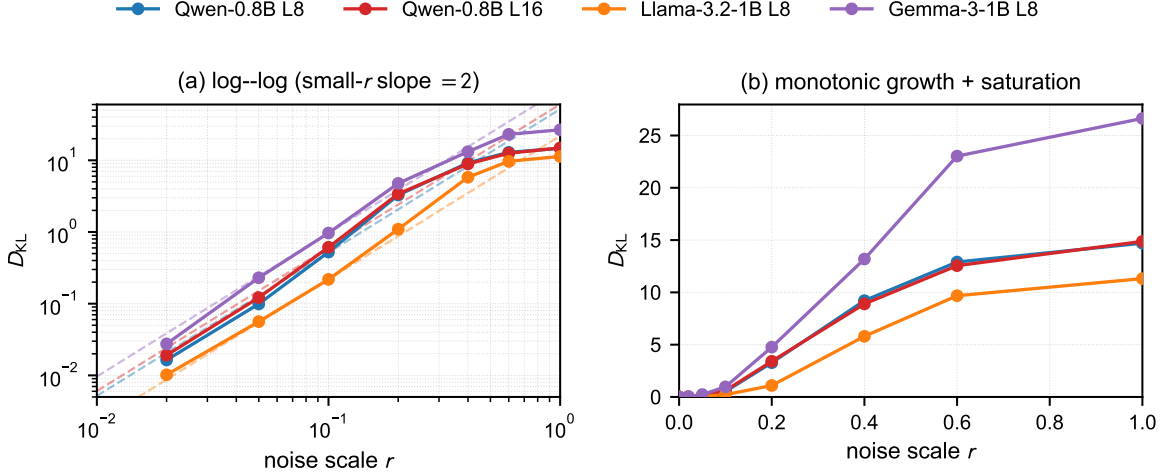
Figure 3: Weight-noise calibration for the open-weight configurations. The mean per-probe next-token KL divergence D_{KL} grows monotonically in the noise scale r , quadratically at small r (consistent with the Fisher-information prediction) and saturating at large r ; on a log-log axis the small-scale regime appears as a slope-2 line. Dashed lines are quadratic fits in the small-scale regime.
