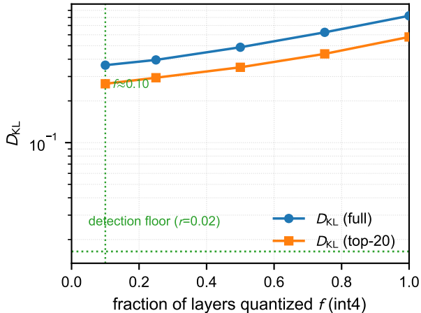
(b) layer-fraction sensitivity (Qwen, L8, int4)
