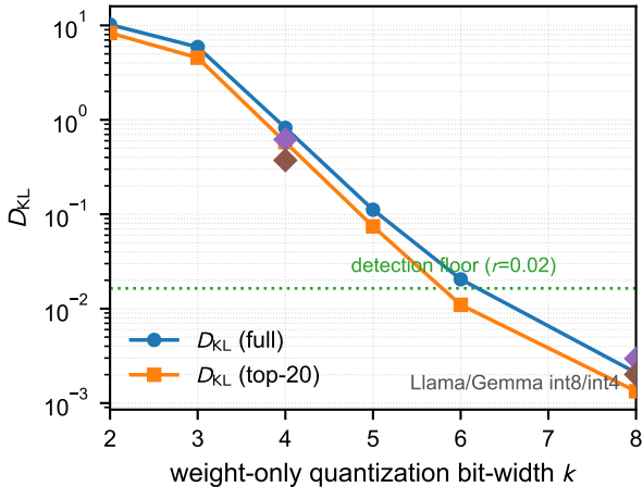
(a) bit-width sensitivity (Qwen, L8)
