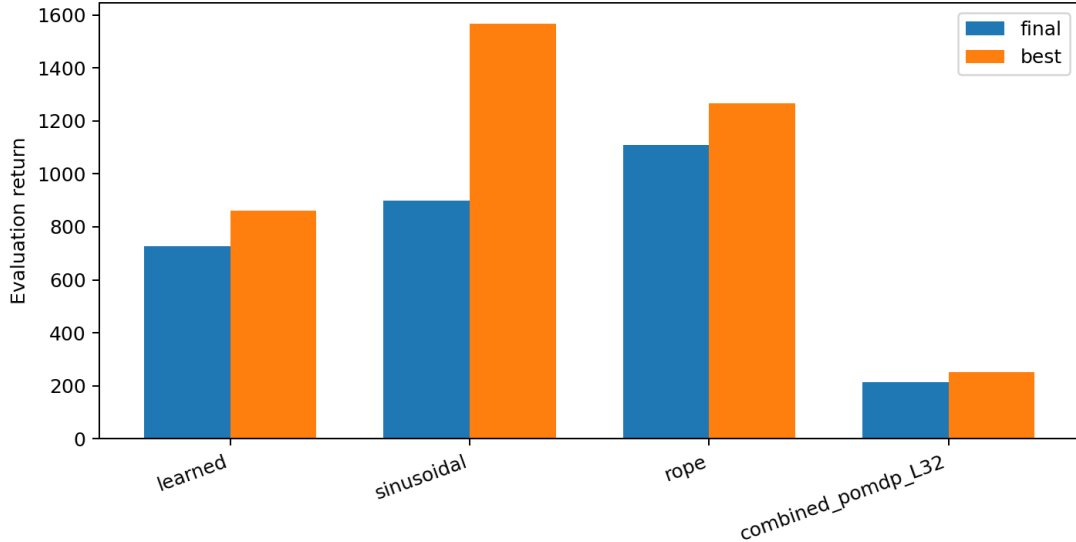
Figure 7: Final and best returns for the newest finished bonus runs counted in this report.
