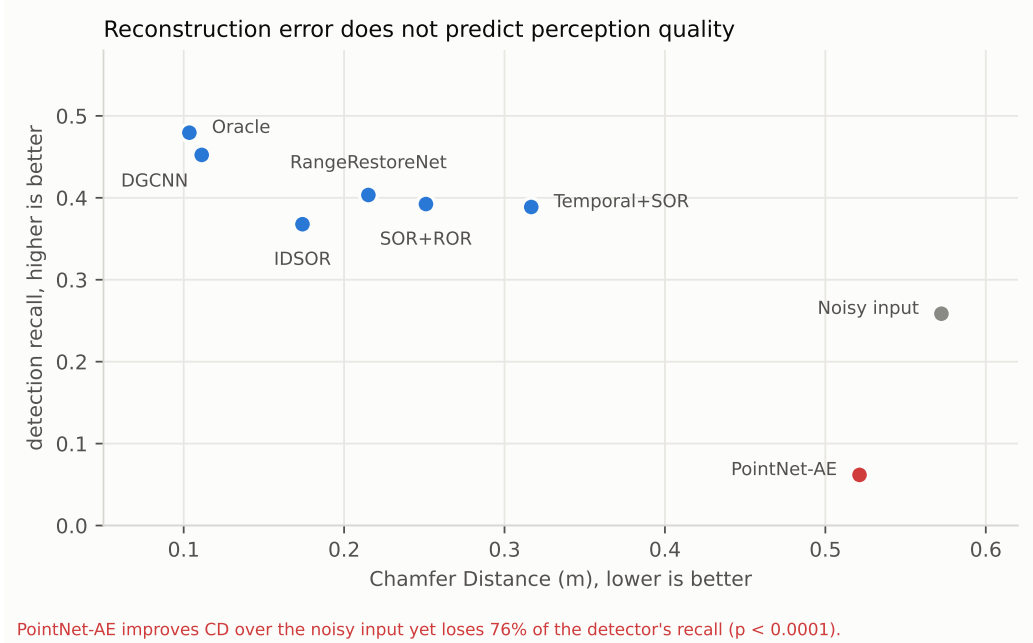
Figure 6: The central result. If Chamfer Distance were a good proxy the methods would lie on a tight descending line. Across all six the rank correlation is only \rho = -0.60 ( p = 0.21 ), directionally right but statistically weak, and the autoencoder is a catastrophic outlier: better CD than the corrupted input, near-zero detection recall. A second, milder inversion is visible in IDSOR, which has clearly better CD than SOR+ROR yet slightly lower recall ( p = 0.069 ).
