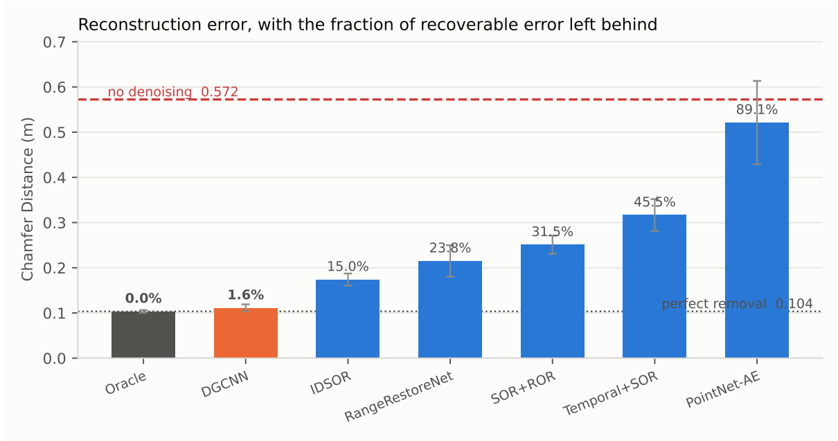
Figure 2: Chamfer Distance by method. Percentages above each bar give the oracle gap. The dotted line is the perfect-removal floor at 0.104 m, non-zero because 31% of returns were destroyed beyond recovery, and the dashed line the uncorrected input. Reading a raw CD against zero rather than against this floor systematically understates every method.
