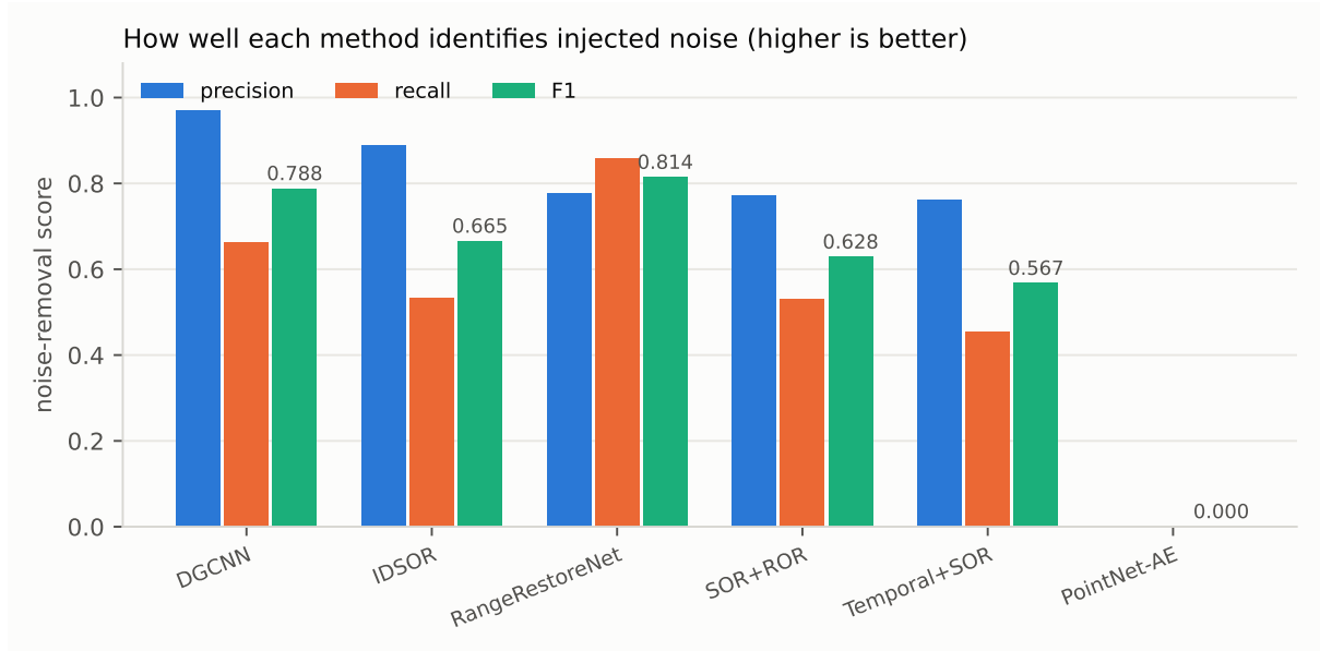
Figure 4: Precision, recall and F1 of noise identification. The two learned classifiers separate along an interpretable axis: the DGCNN is precision-oriented (0.969) and conservative, RangeRestoreNet is recall-oriented (0.859) and aggressive. The autoencoder scores exactly zero because it has no removal head. It is a pure displacement model, which Section 4.3 shows to be actively harmful.
