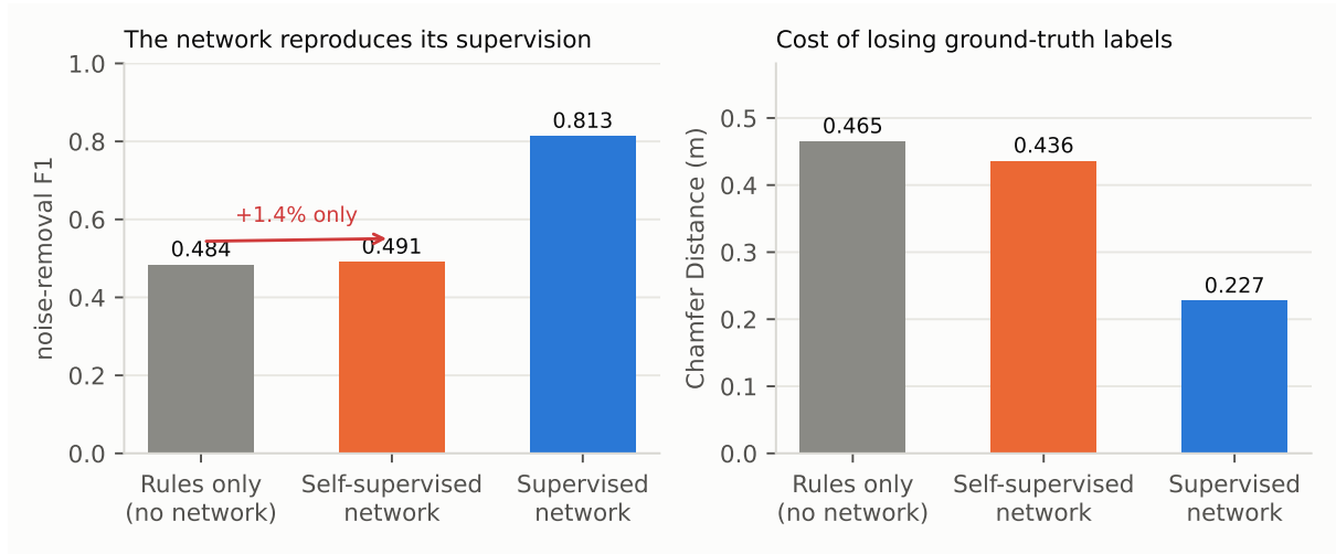
Figure 12: Self-supervision against its own supervision. The pseudo-labels score F1 0.484 against the true labels: roughly half of what the network is told is wrong. Trained on them, the network reaches 60% of the supervised model’s removal F1, but moves F1 only from 0.484 to 0.491.
