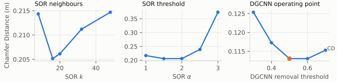
Figure 10: Parameter sensitivity. None of the three parameters is a knife-edge; the DGCNN’s removal threshold in particular is flat between 0.5 and 0.6, so the default is not a tuned artefact.
