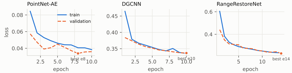
Figure 8: Training and validation loss. The retained checkpoint is the validation minimum, not the final epoch. This is not cosmetic: the autoencoder’s validation loss bottoms at epoch 8 and rises thereafter, so last-epoch selection would have shipped a measurably worse model. The DGCNN’s validation loss was still descending at epoch 10, so its results should be read as a floor on what the architecture achieves rather than a converged ceiling.
