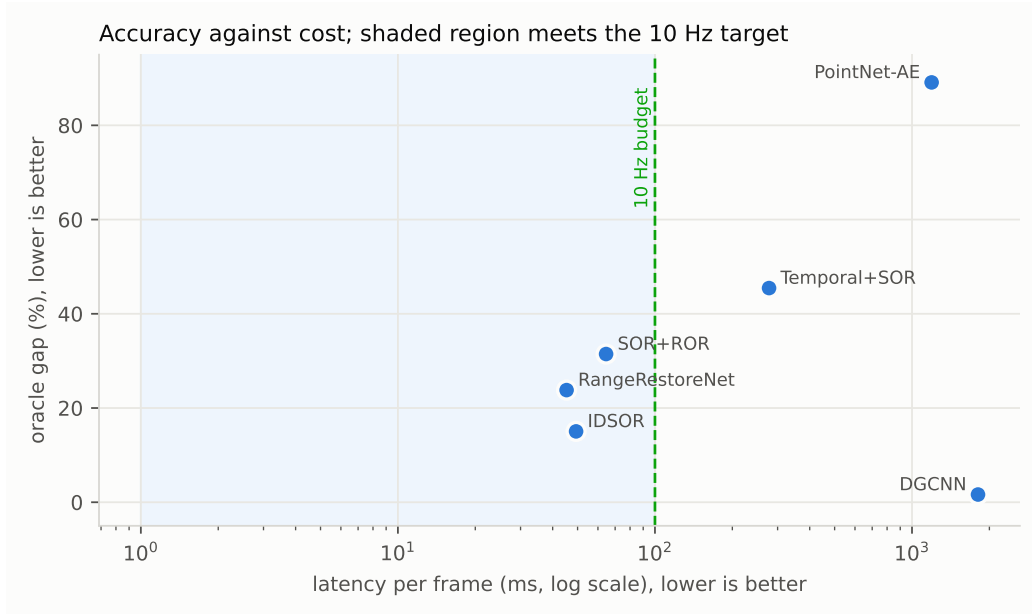
Figure 7: Accuracy against cost. The shaded region meets the 10 Hz target. RangeRestoreNet occupies the position the project needed: within the budget while remaining a learned method.
