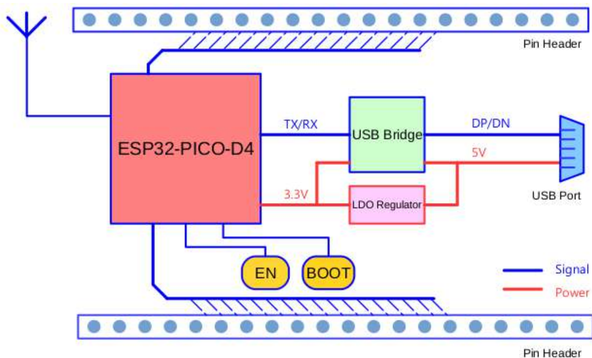
Fig. 33: ESP32-PICO-KIT block diagram
