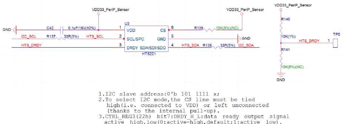
Fig. 20: Temperature and Humidity Sensor Schematics
