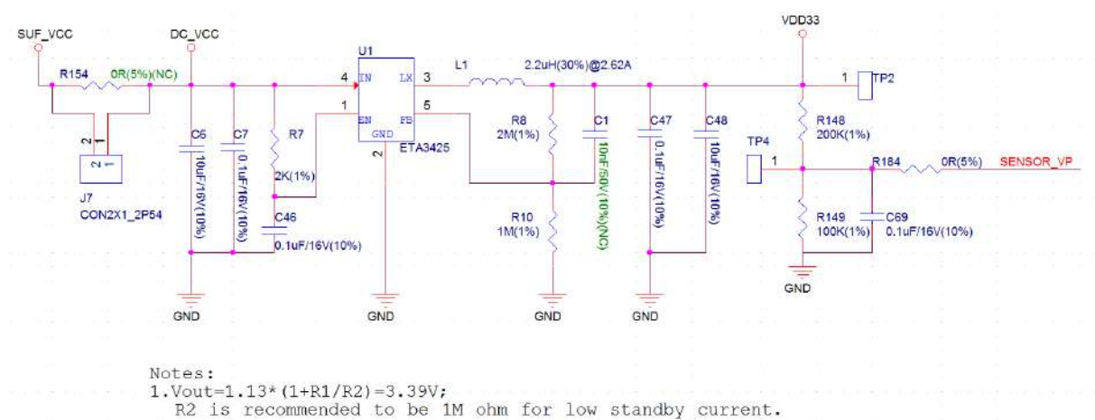
Fig. 14: Peripheral Power Supply Schematics
