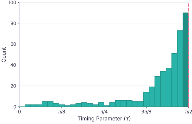
Figure 2. Distribution of optimised timings \tau across the seeds of the LPTE benchmark. Dashed line: \tau = \pi/2 , where the block of Lemma above projects to a maximally entangling SWAP.
