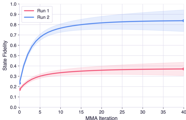
Figure 3. Two representative 8-qubit LPTE optimisation trajectories under triple-channel correlated noise (Run 1: 0.172 \rightarrow 0.371; Run 2: 0.233 \rightarrow 0.838). Shaded bands indicate \pm 1 standard deviation across the 10-seed ensemble.
