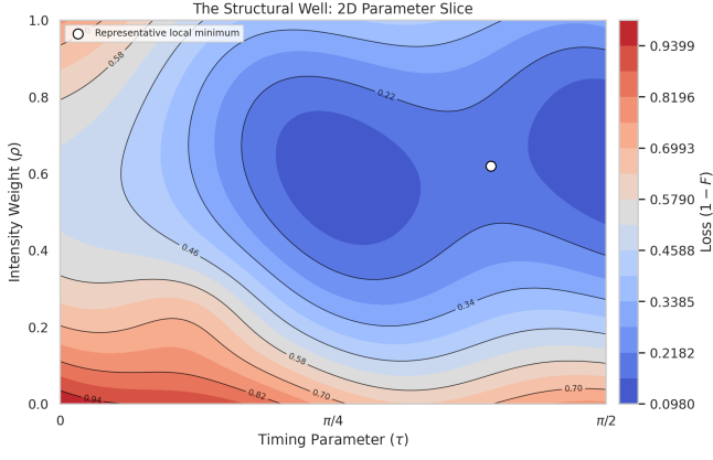
Figure 1. The structural well on FakeFaz, projected onto a 2D (\rho, \tau) slice. Colour encodes the loss L = 1 - F ; solid contours are sublevel sets S_c(L) as defined in Remark 1.
