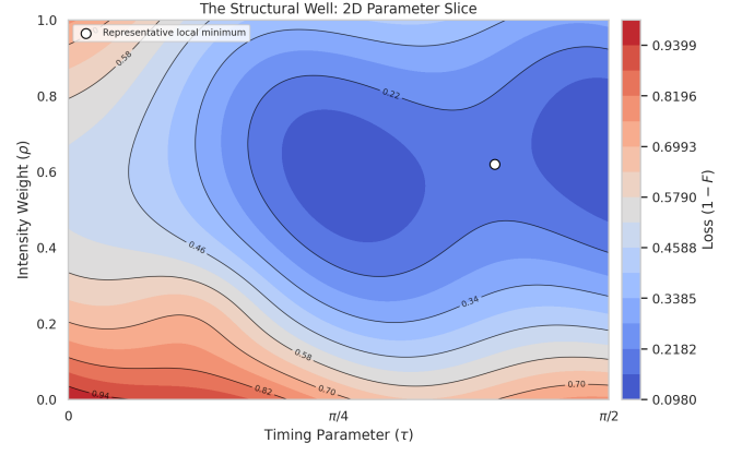
Figure 1. The structural well on FakeFey, projected onto a 2D (\rho, \tau) slice. Colour encodes the loss L = 1 - F ; solid contours are sublevel sets S_c(L) as defined in Remark 1.
