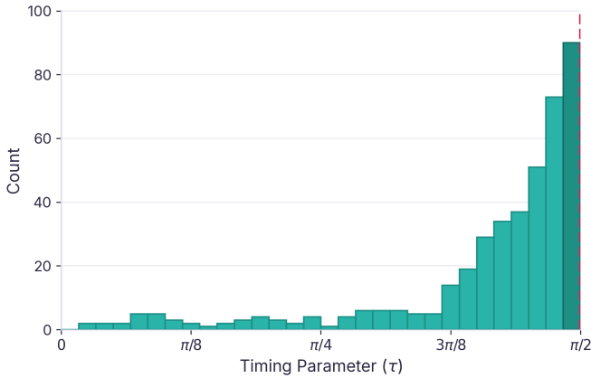
FIG. 2 Distribution of optimised timings \tau across the LPTE benchmark seeds. Dashed line: \tau = \pi/2 , where the block of Lemma 3 projects to a maximally entangling SWAP.
