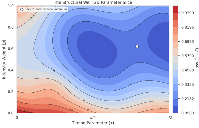
FIG. 1 The structural well on FakeFez, projected onto a 2D (\rho, \tau) slice. Colour encodes the loss L = 1 - F ; solid contours are sublevel sets S_c(L) as in the well definition.
