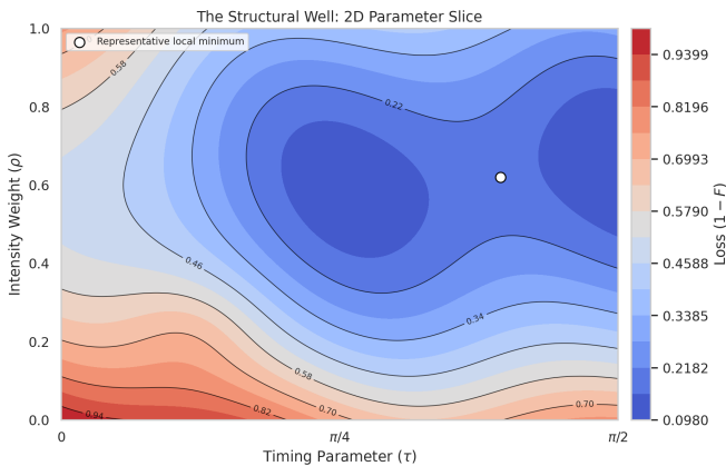
FIG. 1 The structural well on FakeFcz, projected onto a 2D (\rho, \tau) slice. Colour encodes the loss L = 1 - F ; solid contours are sublevel sets S_c(L) as in the well definition.
