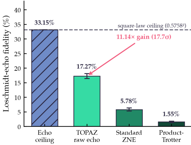
FIG. 6 Live ibm_fez Loschmidt echo: TOPAZ raw echo versus product-Trotter baseline and standard ZNE, against the square-law ceiling of Eq. (9). The hatched bar is a theoretical bound, not a measurement.
