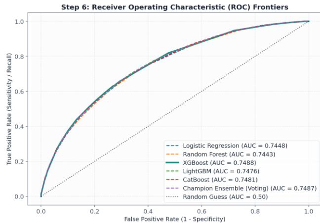
Fig. 1. Out-of-time Receiver Operating Characteristic (ROC) curves across all benchmark models on holdout test data.
