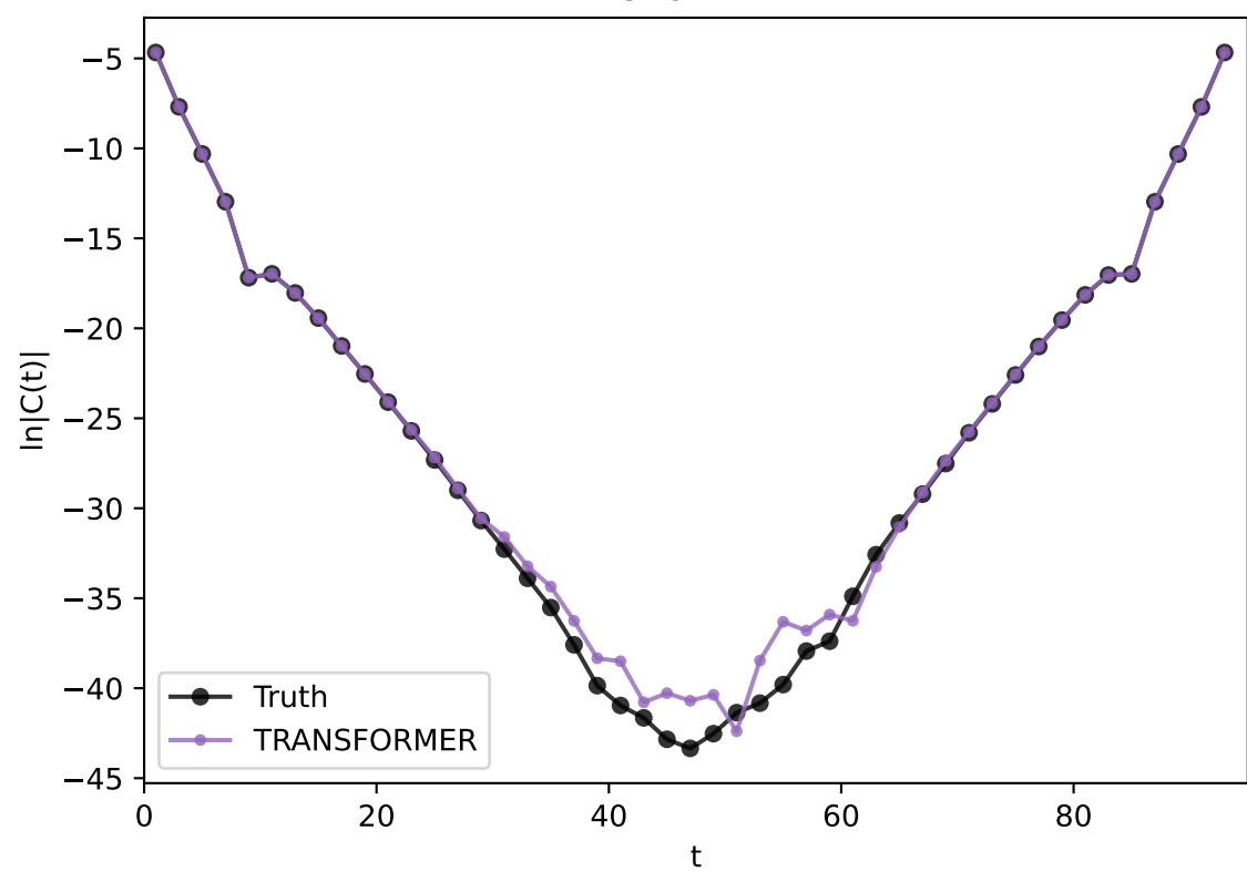
TRANSFORMER: RM
