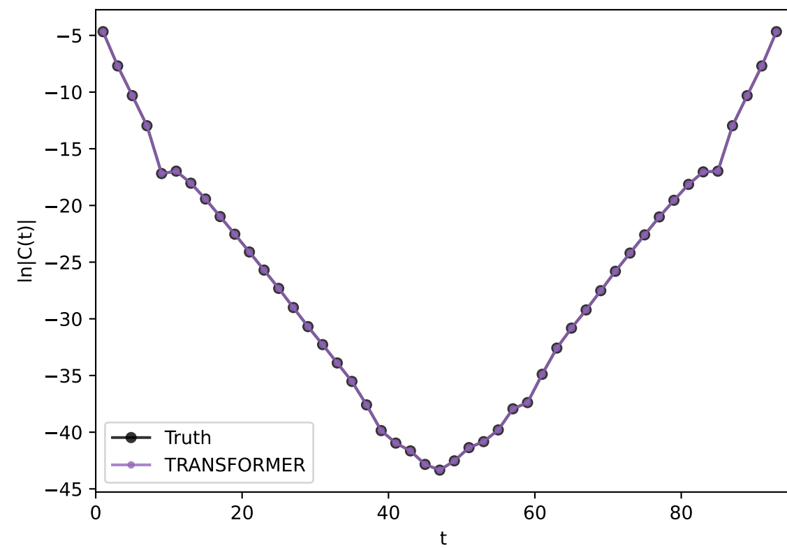
TRANSFORMER: BC
