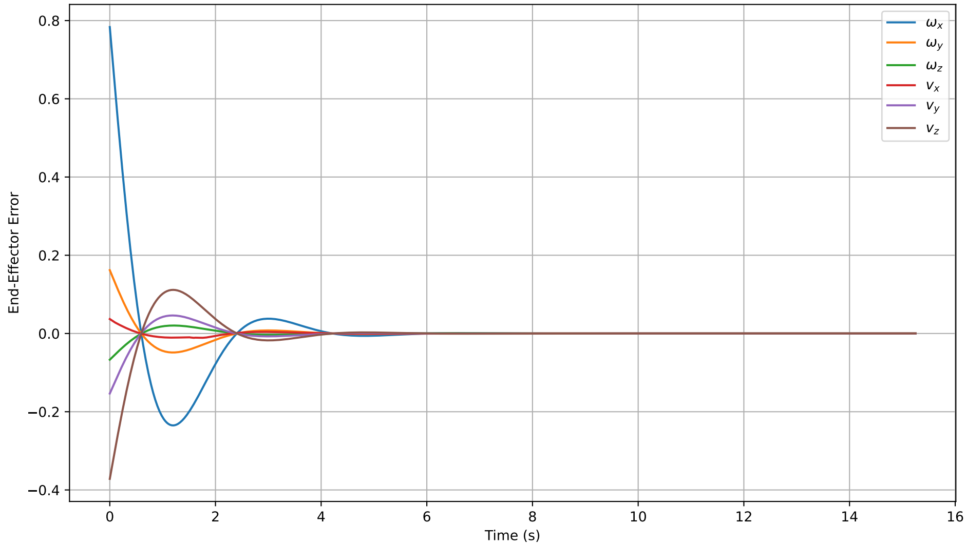
End-Effector Tracking Error — overshoot
