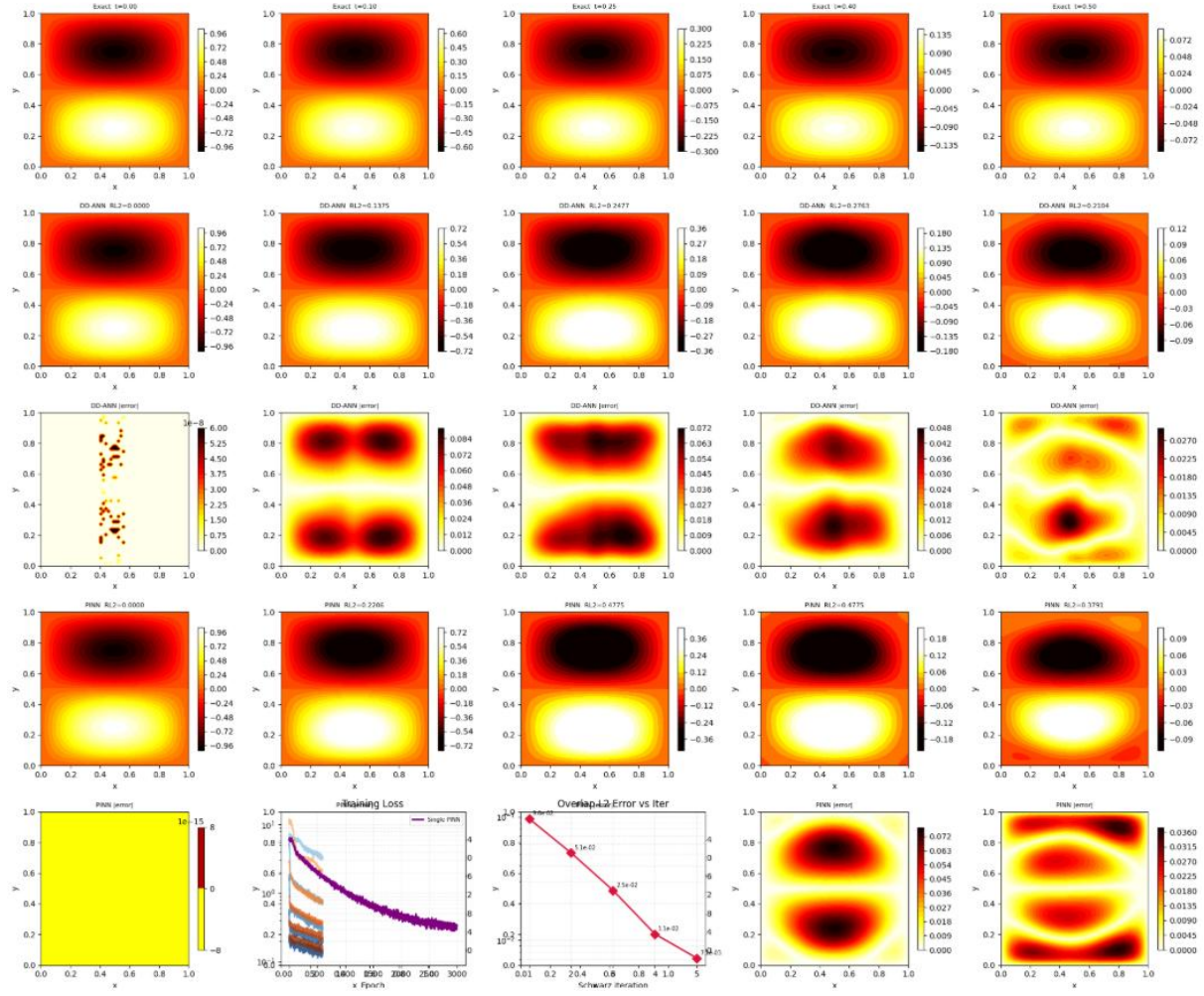
P2: Higher Mode u = \exp(-5\pi i 2t) \sin(\pi x) \sin(2\pi y) DD-ANN 90.2s vs Single PINN 48.3s
