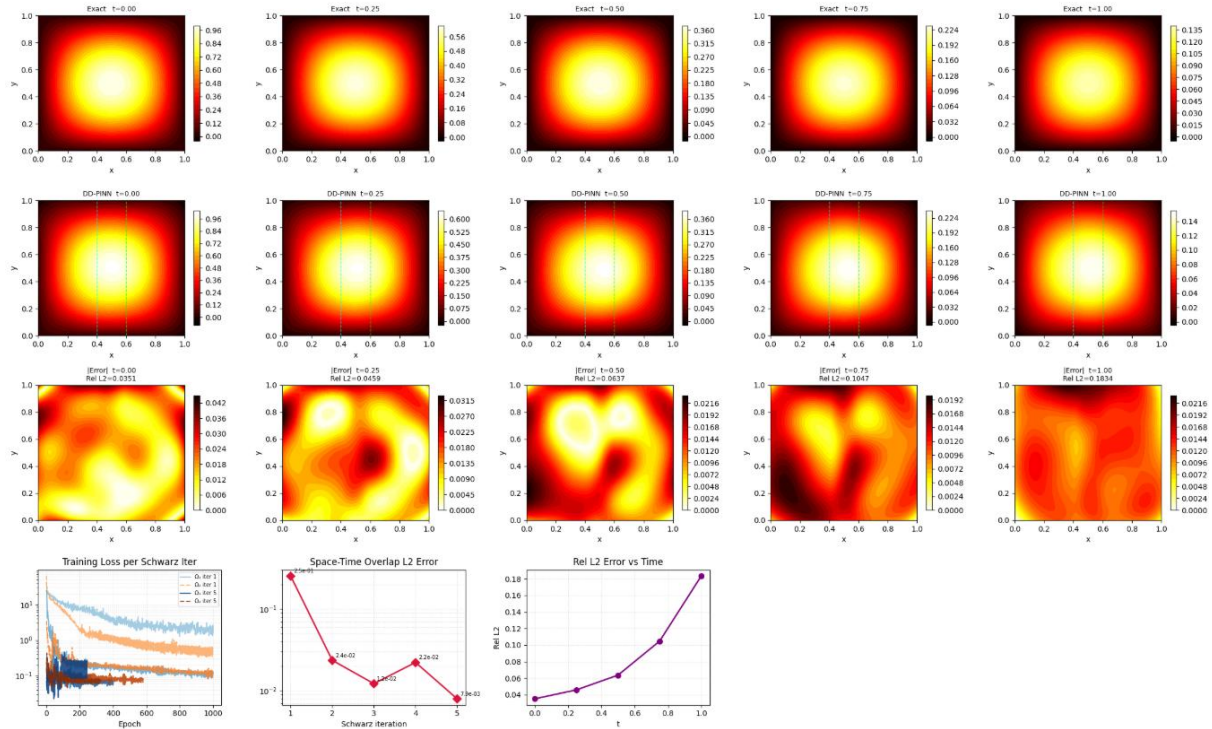
Problem 1: Single Decaying Mode | Overlap [0.4,0.6] | Time: 162.83s
