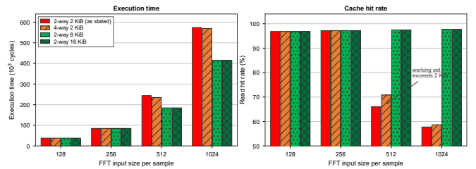
Fig. 1. FFT execution time and read hit rate against problem size for four cache configurations. The two 2 KiB configurations diverge from the two larger ones exactly where the working set stops fitting, and doubling associativity does not close the gap. The 8 KiB and 16 KiB curves coincide at every point.
