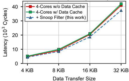
MemLat 2 (on-chip BRAM)
