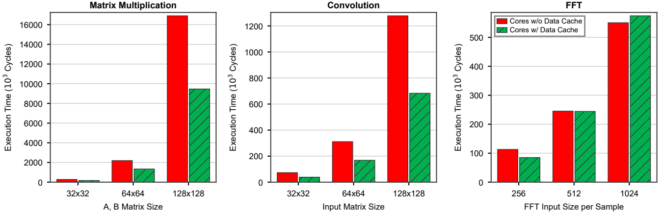
Fig. 2. Execution time against problem size for the three benchmark kernels, with and without the data cache, on the axes of the original’s own execution-time figure so the two may be read against each other directly. Matrix multiplication and convolution reproduce the \approx 40\% reduction it reports. FFT reproduces its \approx 23\% only at N=256 : the benefit falls to 0.4\% at 512 and is negative at 1024, where a 2 KiB DCU no longer holds the 8N -byte per-PE working set and the cache costs more than it saves. Regenerated by scripts/plot_fig6.py from results/fig6.csv .
