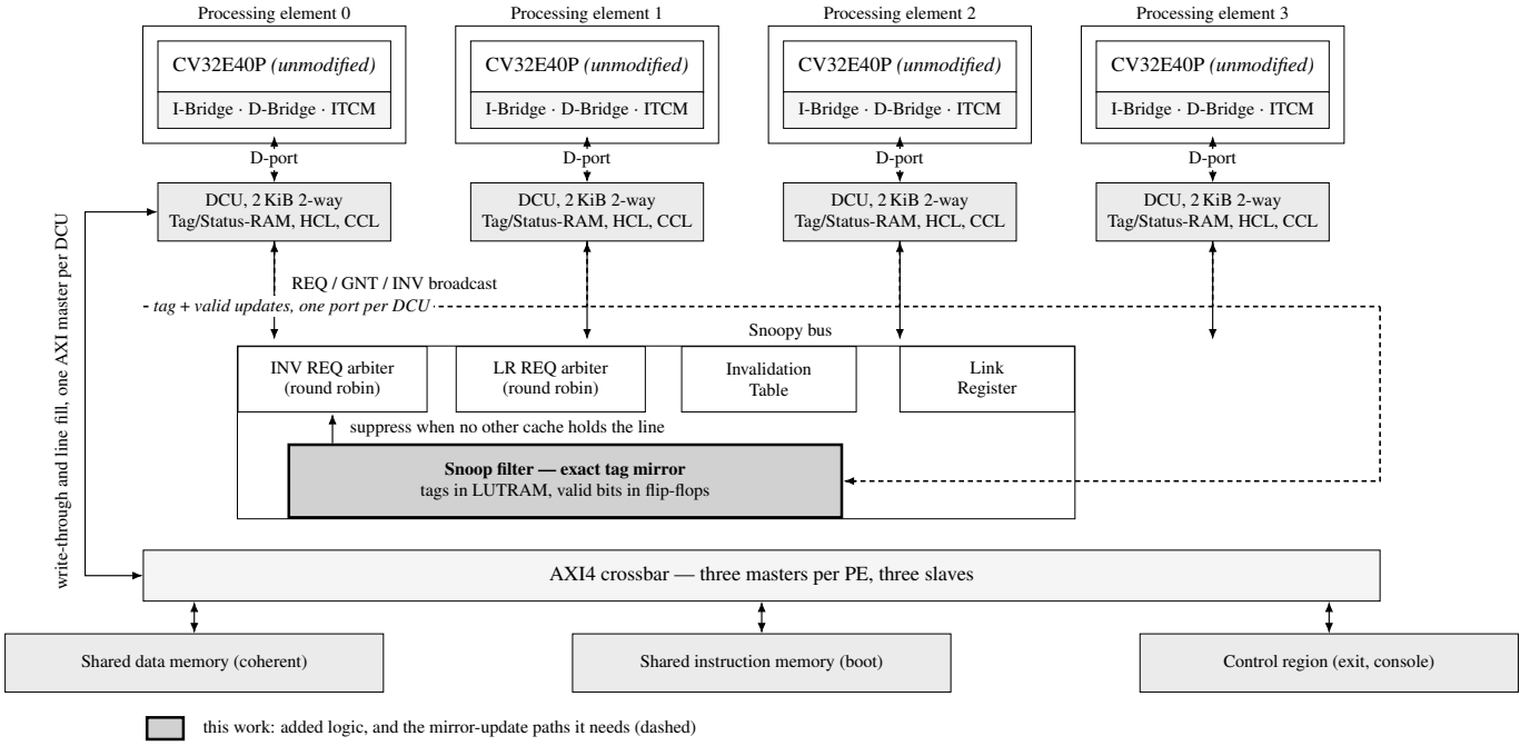
Fig. 1. Overview of the multi-core RISC-V architecture with the cache extension of [1] and the snoop filter added by this work (shaded). The filter holds a mirror of the tag and valid bits of every DCU and tells the INV REQ arbiter whether any other DCU has to receive the request.
