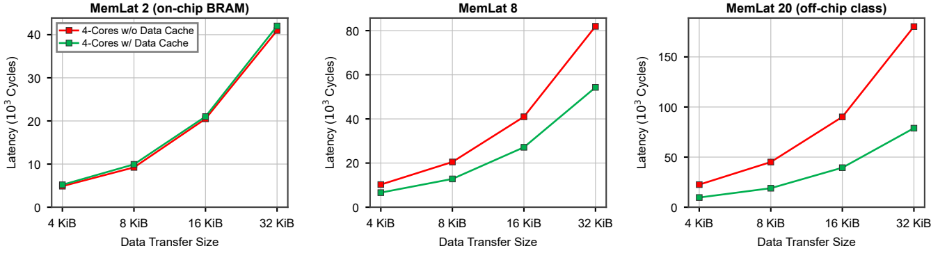
Fig. 3. Memory-copy latency against transfer size, with and without the data cache, on the axes of the original’s Fig. 5. Whether its \approx 50\% reduction reproduces depends entirely on how slow the shared memory is, which its text does not state. At a memory latency of two – a block RAM answering almost immediately – the extension is 2.5 to 7.6% slower than no cache at all, because a streaming kernel has no reuse against which to amortise a line fill. At twenty it is 56 to 58% faster, which is close to the reported figure. Regenerated by scripts/plot_fig5.py from results/fig5.csv .
