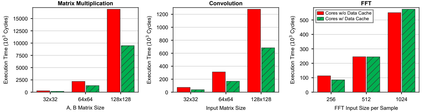
Fig. 2. Execution time against problem size for the three benchmark kernels, with and without the data cache, on the axes of the original’s own execution-time figure so the two may be read against each other directly. Matrix multiplication and convolution reproduce the \approx 40\% reduction it reports. FFT reproduces its \approx 23\% only at N=256 ; the benefit falls to 0.4\% at 512 and is negative at 1024, where a 2 KiB DCU no longer holds the 8N -byte per-PE working set and the cache costs more than it saves. Regenerated by scripts/plot_fig6.py from results/fig6.csv .
