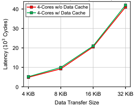
MemLat 2 (on-chip BRAM)
