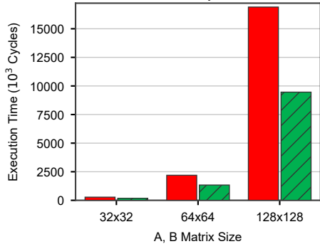
Matrix Multiplication
