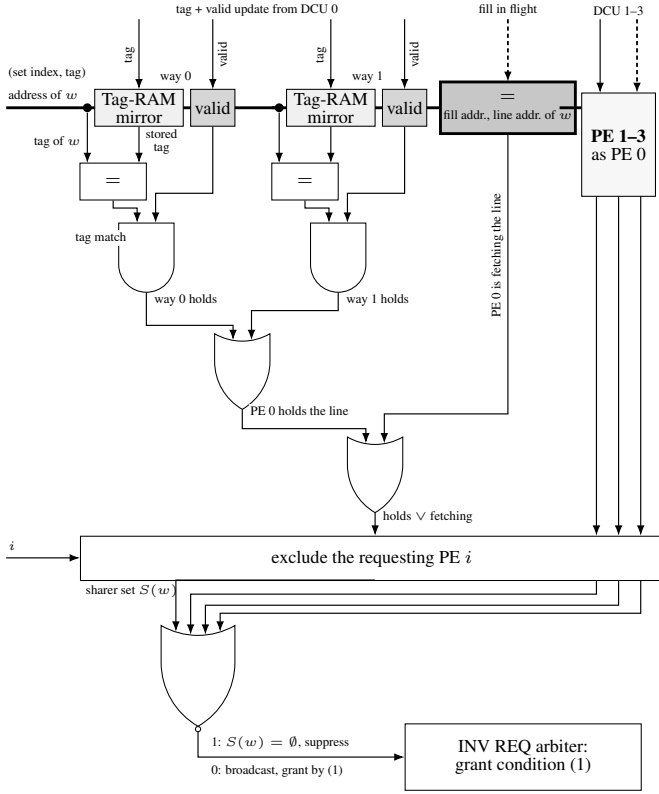
Fig. 2. Decision path of the snoop filter for the INV REQ selected by the INV REQ arbiter, issued by PE i with address of w . The address bus reads every Tag-RAM mirror and valid bit at its set index; per way, a comparator matches the stored tag against the tag of w and an AND gate qualifies it with the valid bit; the two ways are ORed, then ORed with the fill comparator of Section V-B (shaded). PE 1–3 are identical. Excluding PE i gives the sharer set S(w) , and a NOR over its bits decides whether the broadcast is suppressed.
