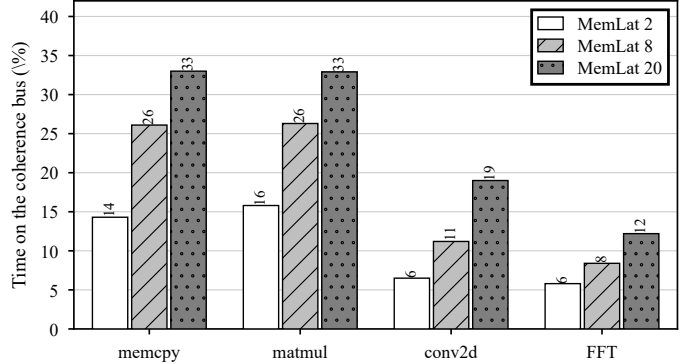
Fig. 2. Time each core spends waiting for a snoop-bus grant, as a percentage of the cycles it had an access in the DCU. Table II shows that none of the traffic it is waiting for is necessary.
