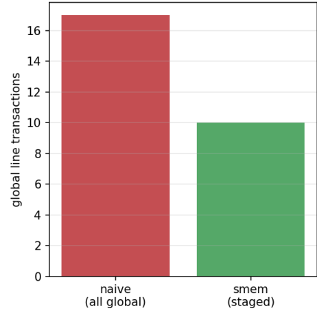
Fig. 4. Global line transactions for an 8\times 8 matmul row: staging the reused row in the scratchpad cuts off-chip traffic.
