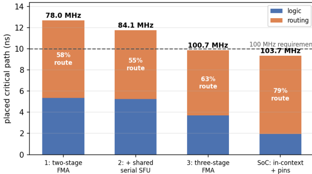
Fig. 11. Placed critical path at each closure step, split into logic and routing delay (worst path of each sign-off timing report; achieved Fmax above each bar). Every step is routing-dominated: the three-stage FMA closes timing by shortening the whole cone, not by reducing the wire share, which rises to 79% in the deployable SoC.
