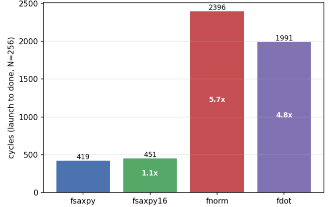
Fig. 9. Cycles at N=256 for the FP application kernels. The multi-cycle divide/square-root SFU makes f_{\text{norm}} about 6 \times the streaming f_{\text{saxpy}} ; f_{\text{dot}} pays for its scratchpad reduction.
