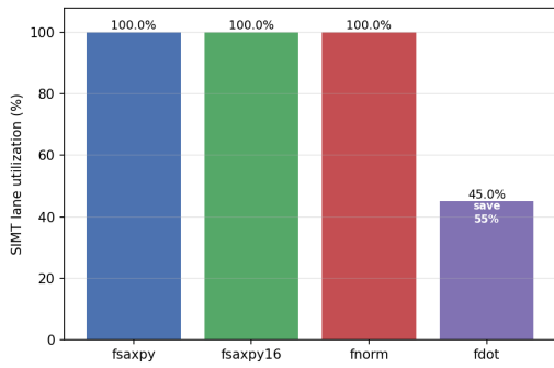
Fig. 10. SIMT lane utilization per FP kernel. Streaming kernels keep all lanes busy; fdot ’s single-lane reduction idles 55% of the (now FP-enlarged) lane datapath, which mask-driven clock-gating removes.
