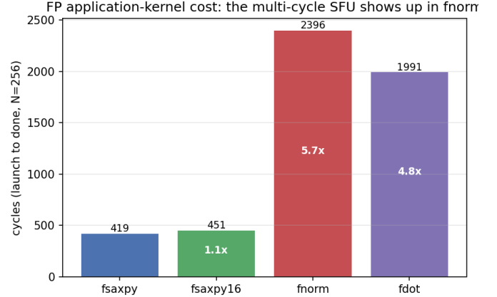
Fig. 9. Cycles at N=256 for the FP application kernels. The multi-cycle divide/square-root SFU makes f_{\text{norm}} about 6 \times the streaming f_{\text{saxpy}} ; f_{\text{dot}} pays for its scratchpad reduction.
