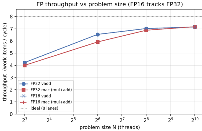
Fig. 2. Floating-point throughput versus problem size for streaming add and multiply-add kernels. The ramp is the same latency-hiding behavior as the integer suite; the FP16 curves coincide with the FP32 ones because both use the same pipelined datapath.
