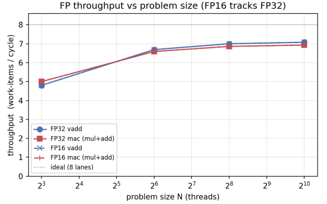
Fig. 7. Floating-point throughput versus problem size for streaming add and multiply-add kernels. The ramp is the same latency-hiding behavior as the integer suite; the FP16 curves coincide with the FP32 ones because both use the single-cycle datapath.
