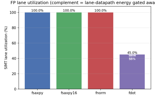
Fig. 10. SIMT lane utilization per FP kernel. Streaming kernels keep all lanes busy; fdot ’s single-lane reduction idles 55% of the (now FP-enlarged) lane datapath, which mask-driven clock-gating removes.
