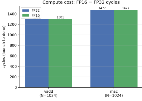
Fig. 8. Cycles to completion at N=1024 : FP16 equals FP32 for both kernels, confirming half precision adds no compute-time cost on the single-cycle FP unit.
