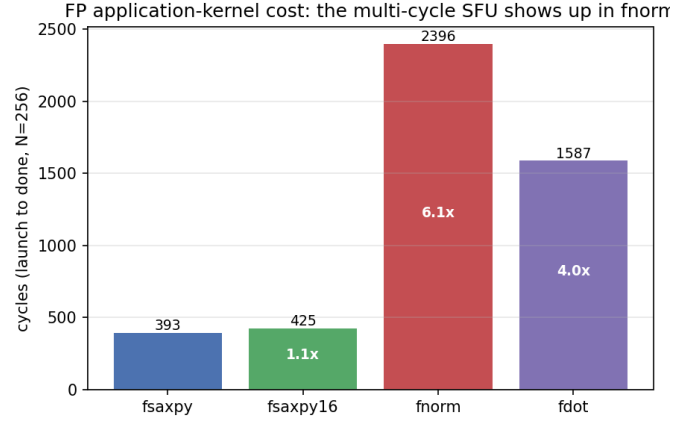
Fig. 9. Cycles at N=256 for the FP application kernels. The multi-cycle divide/square-root SFU makes fnorm about 6× the streaming fsaxpy ; fdot pays for its scratchpad reduction.
