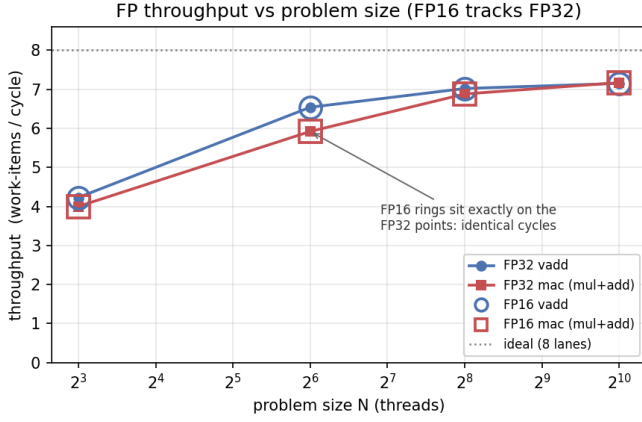
Fig. 7. Floating-point throughput versus problem size for streaming add and multiply-add kernels. The ramp is the same latency-hiding behavior as the integer suite; the hollow FP16 markers sit exactly on the FP32 curves because both use the same pipelined datapath.
