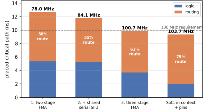
Fig. 3. Placed critical path at each closure step, split into logic and routing delay (worst path of each sign-off timing report, with the achieved F_{\max} above each bar). Every step is routing-dominated.
