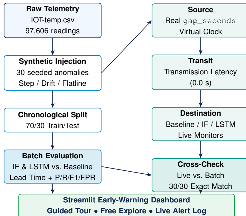
Figure 5.1: Digital-Twin-Integrated Early Warning System Architecture: the offline batch pipeline (left) trains and evaluates both detectors; the SimPy digital twin (right) replays the same stream live with both detectors wired in as monitors; a cross-check confirms the two never diverge.
