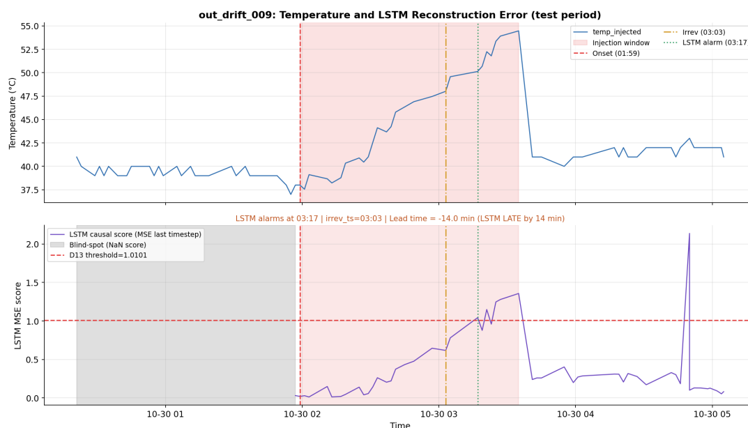
Figure 6.3: The one case where the LSTM-Autoencoder is measurably late: out_drift_009. The reconstruction-error score crosses its threshold only after irreversibility onset (14.0 minutes late), illustrating that a reconstruction-based detector can lag a fast-accelerating drift even when its score does eventually respond correctly.
