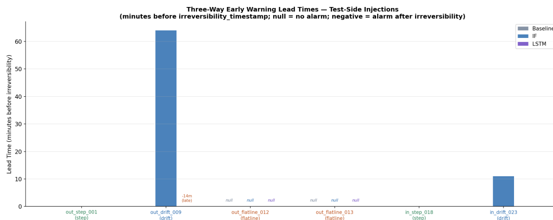
Figure 6.1: Early-warning lead time by detector across the six test-side injections. Isolation Forest is the only detector to beat the naive baseline, on both drift injections; neither detector improves on the baseline for either step or either flatline injection.
