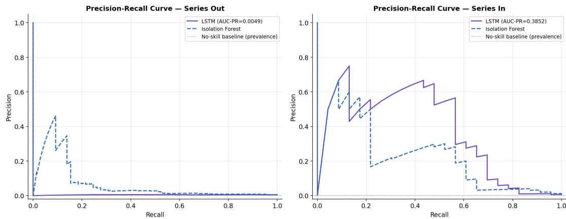
Figure 6.2: Precision-recall curves, Isolation Forest vs. LSTM-Autoencoder, both series. The LSTM-Autoencoder dominates on the In series (AUC-PR 0.385 vs. 0.237) but is essentially at chance on the Out series (AUC-PR 0.005 vs. IF's 0.068).
