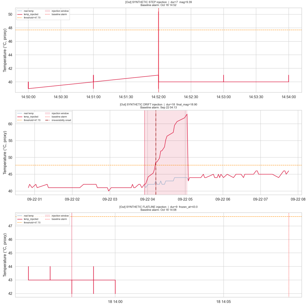
Figure 5.3: Representative synthetic step, drift, and flatline injections on the Out series, explicitly labelled as synthetic stress-test events, never presented as real found anomalies.
