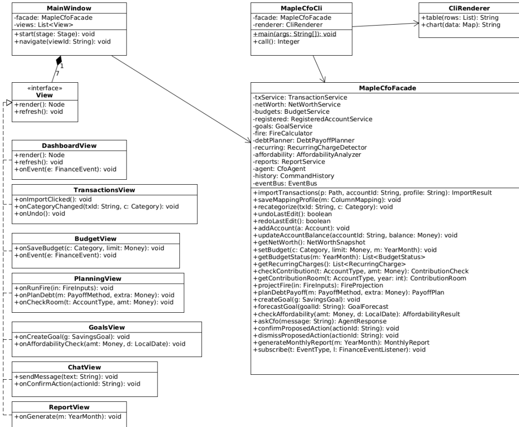
Class diagram (6/6): Presentation, Facade and persistence (Facade, MVC, Repository/DAO)
