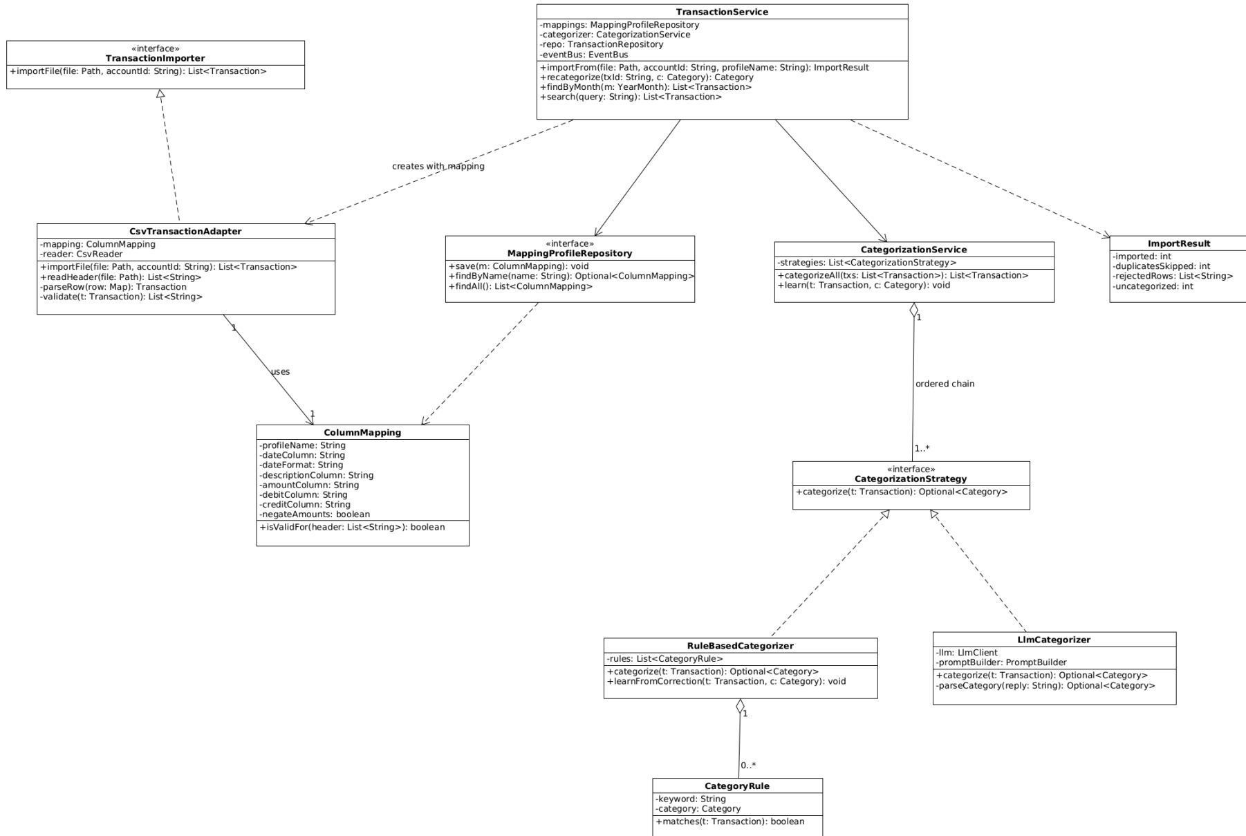
Class diagram (2/6): Import and categorization (Adapter, Strategy)
