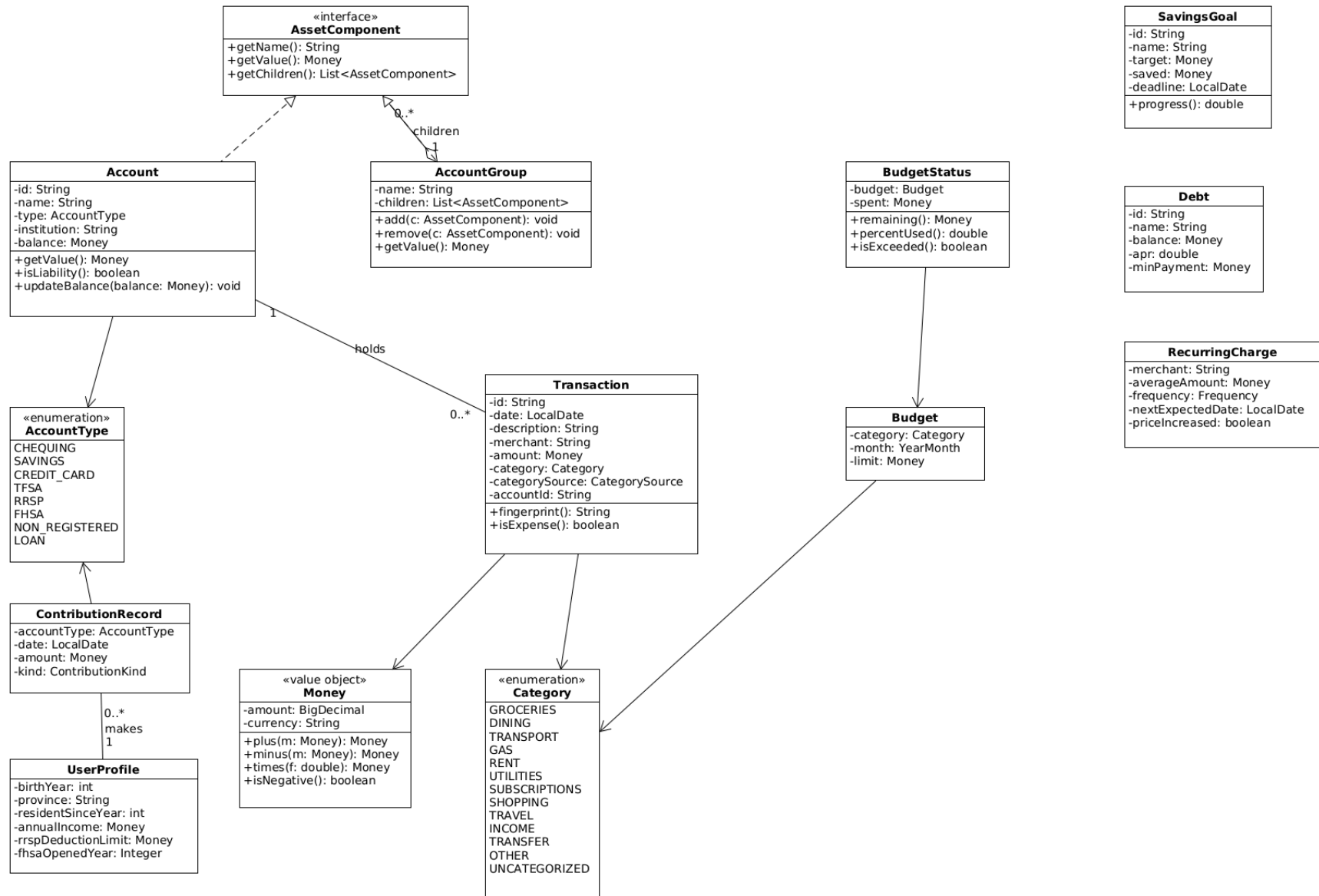
Class diagram (1/7): Domain model (Composite: net worth)
