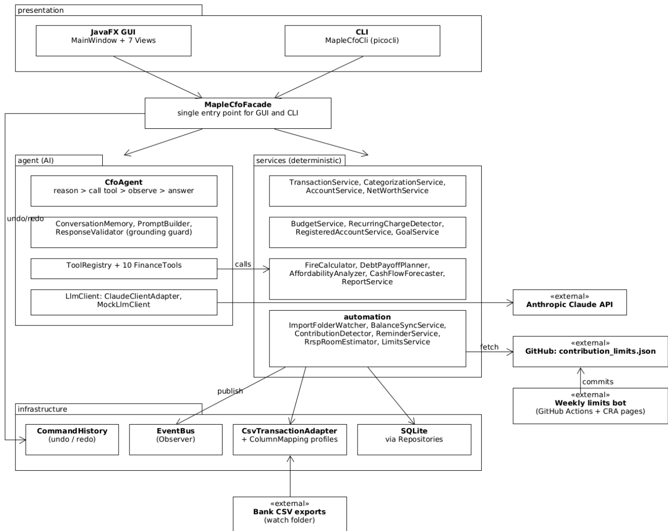
Architecture: layered package view
