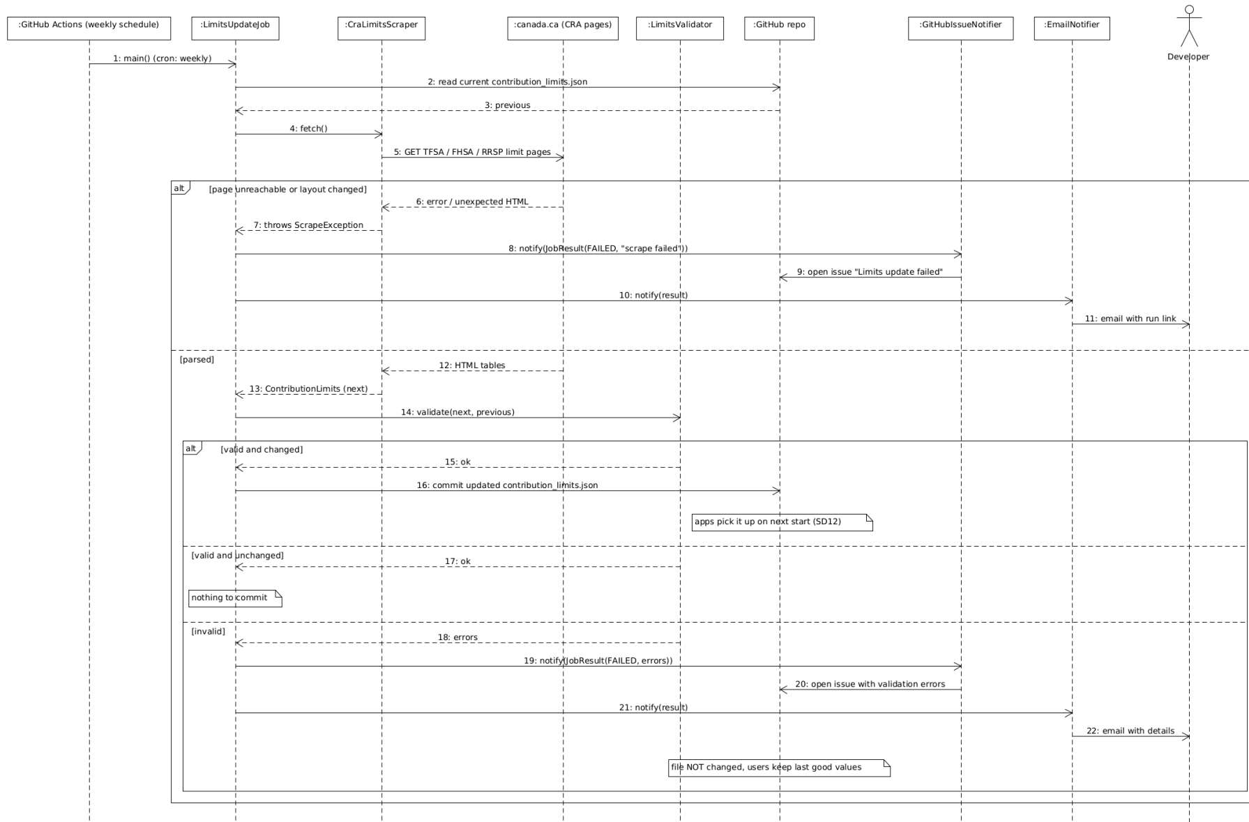
SD13: Weekly limits bot with failure alerts (F15)
