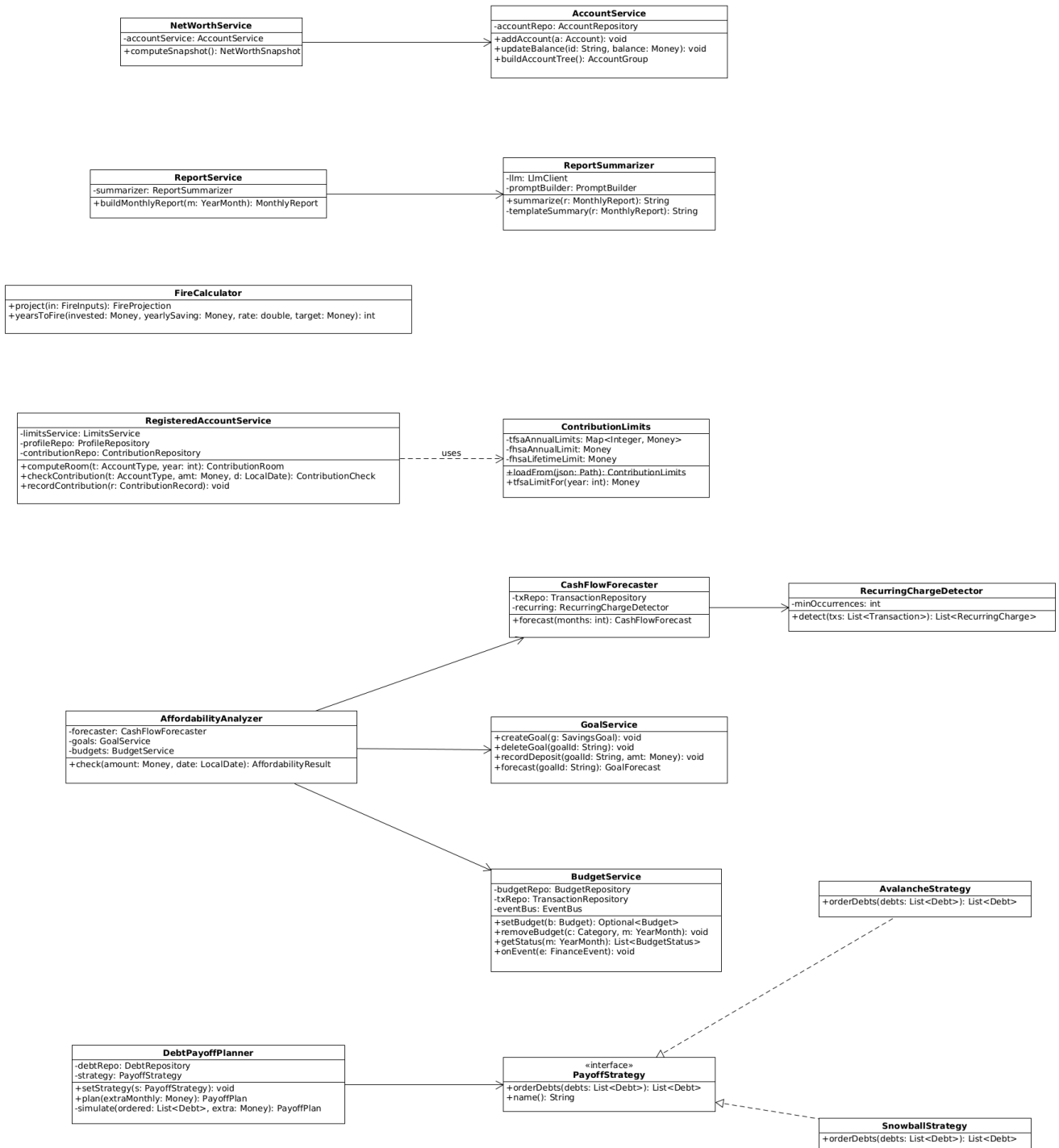
Class diagram (3/7): Planning and analysis services (Strategy)
