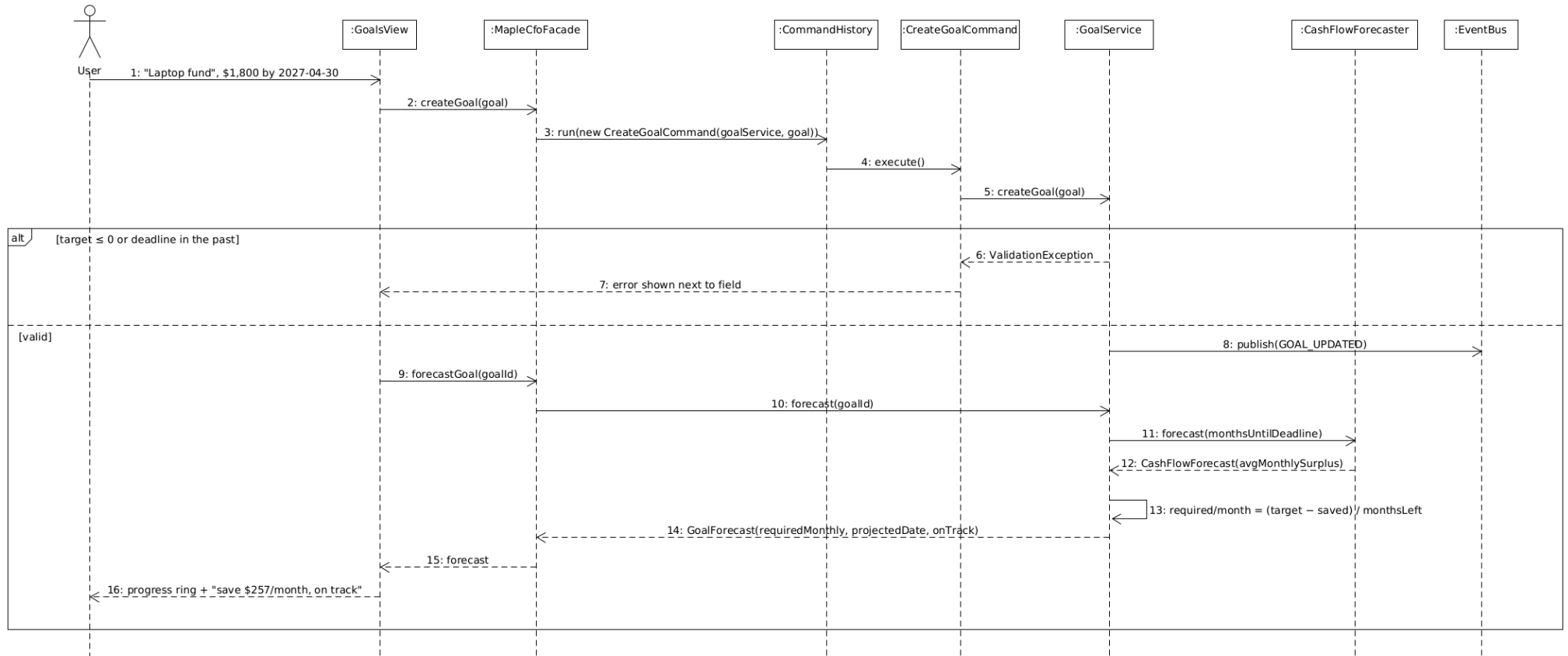
SD07: Create and forecast a savings goal (F09)
