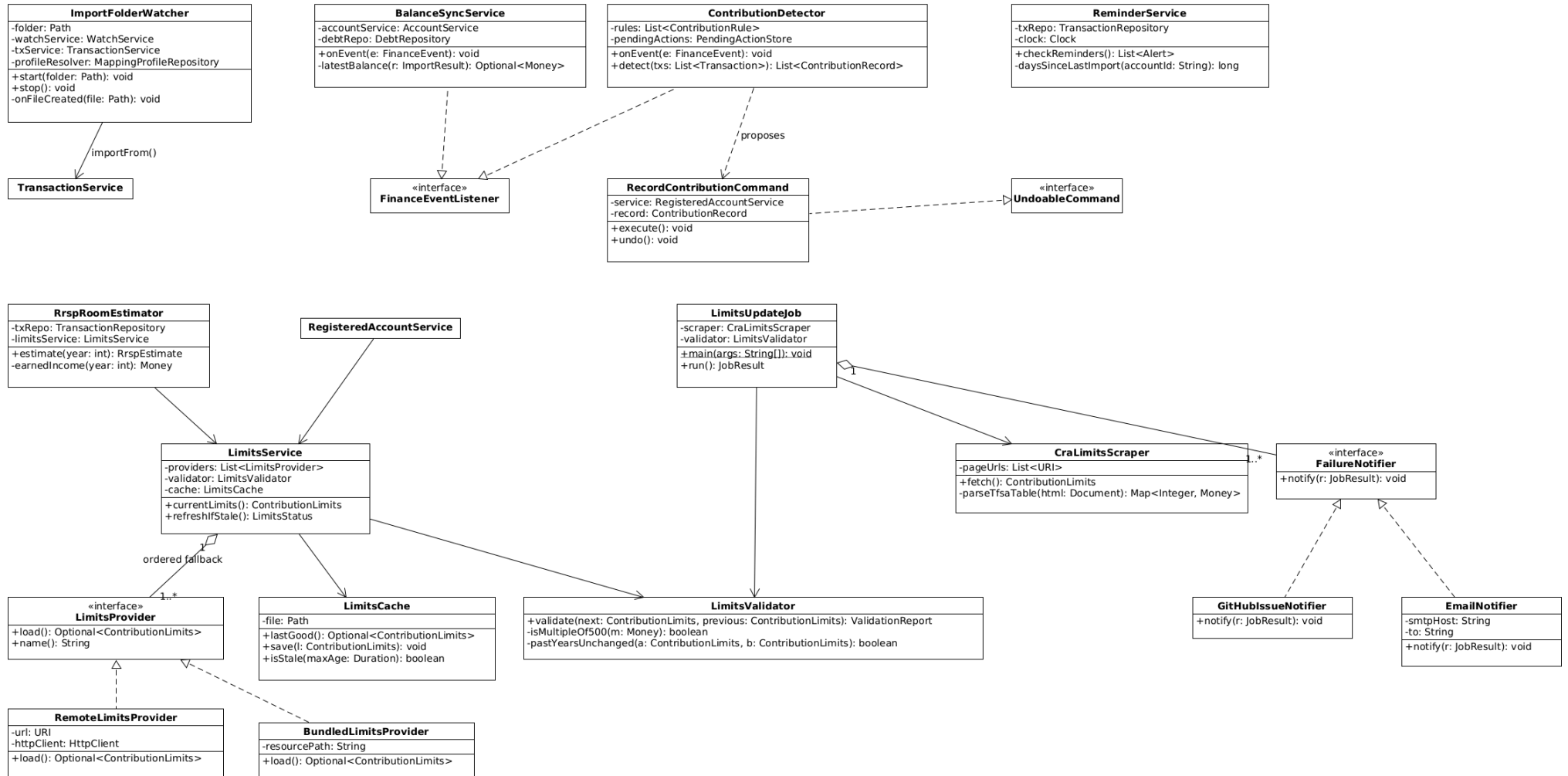
Class diagram (7/7): Automation (auto-sync, contribution detection, self-updating limits)
