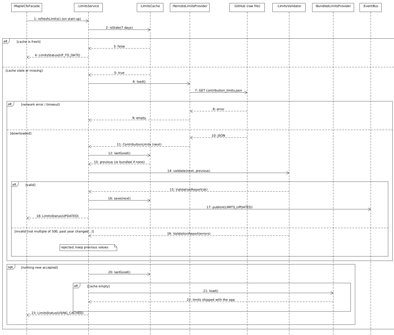
SD12: App start-up, self-updating contribution limits with fallback (F15)
