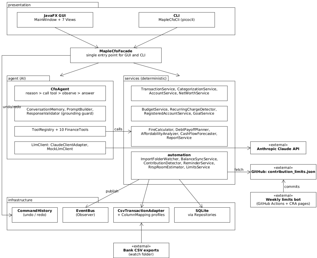
Architecture: layered package view
