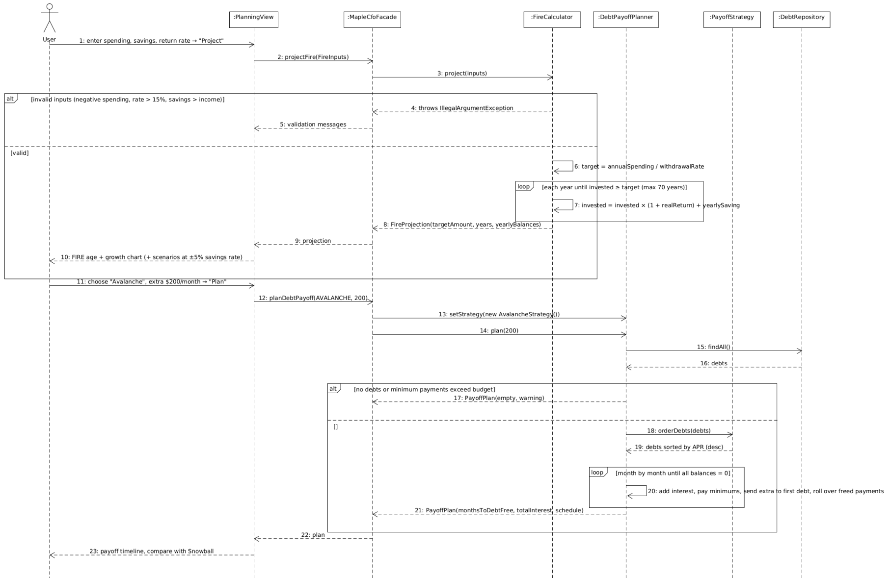
SD05: FIRE projection and debt payoff plan (F07, F08)
