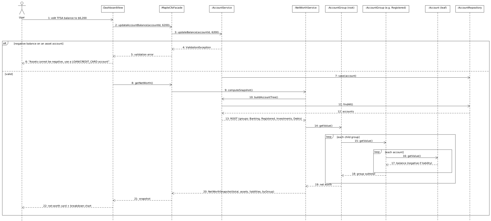
SD03: Update an account and view net worth (F03)
