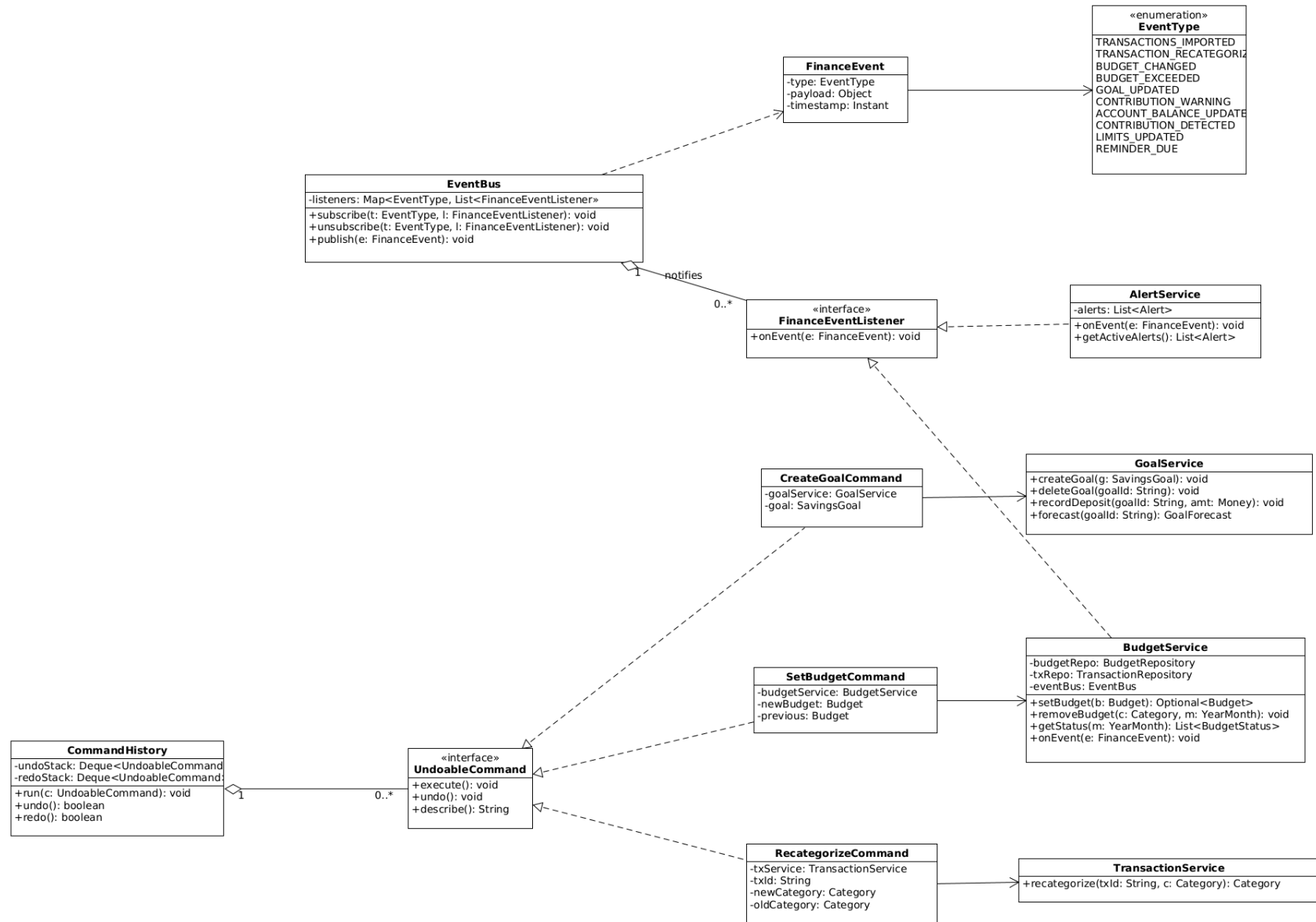
Class diagram (4/7): Events and undoable commands (Observer, Command)
