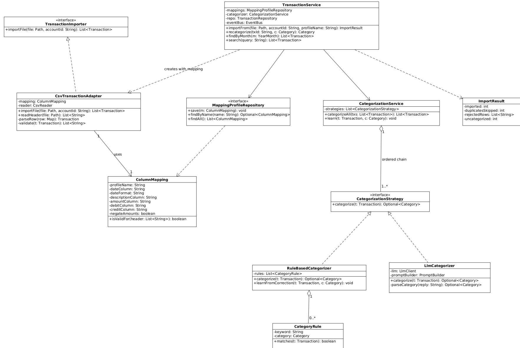
Class diagram (2/7): Import and categorization (Adapter, Strategy)
