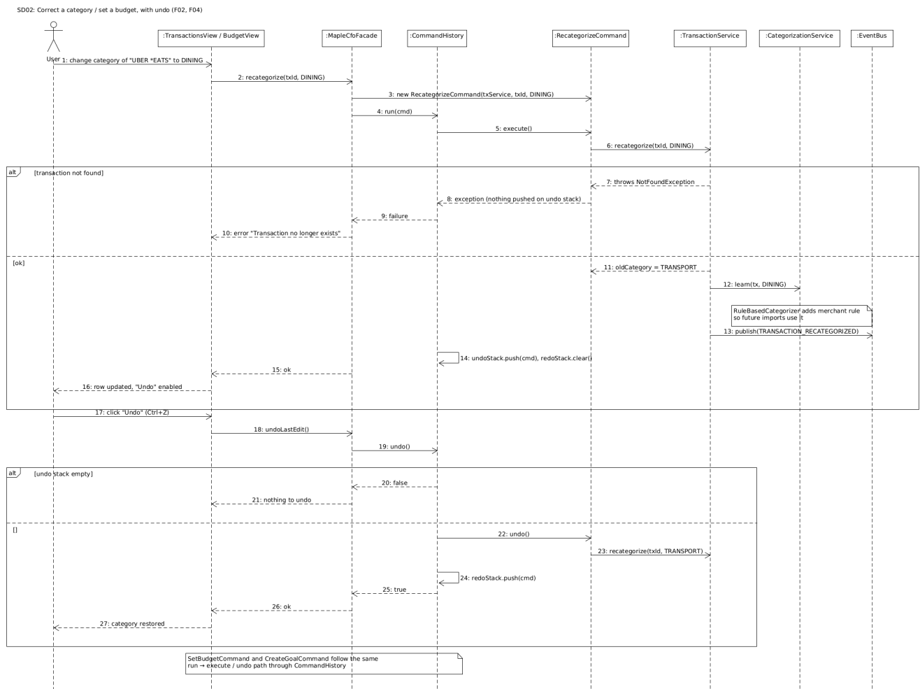
SD02: Correct a category / set a budget, with undo (F02, F04)
