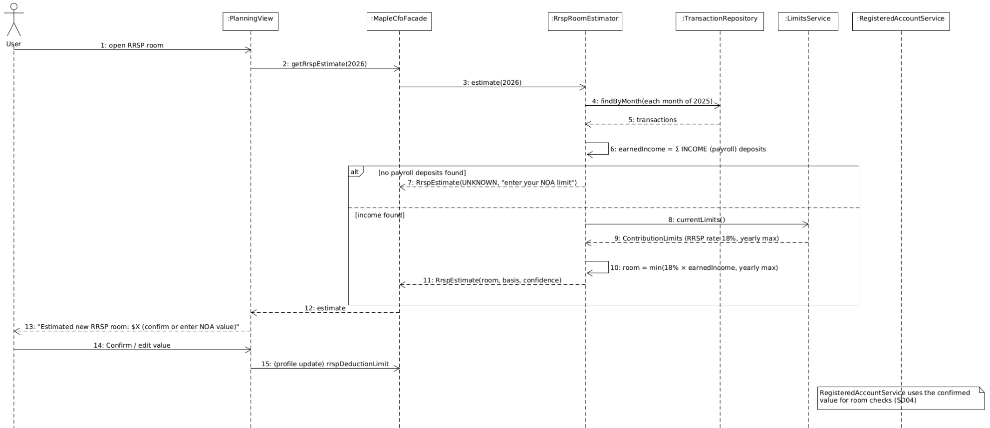
SD14: RRSP room estimate from payroll deposits (F14)
