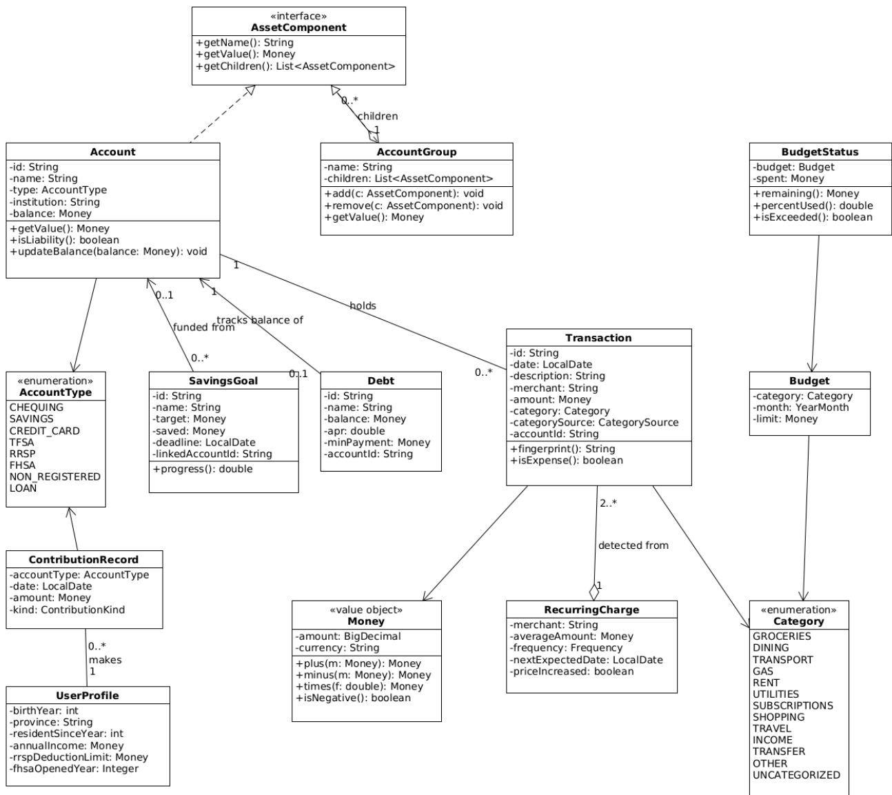
Class diagram (1/7): Domain model (Composite: net worth)
