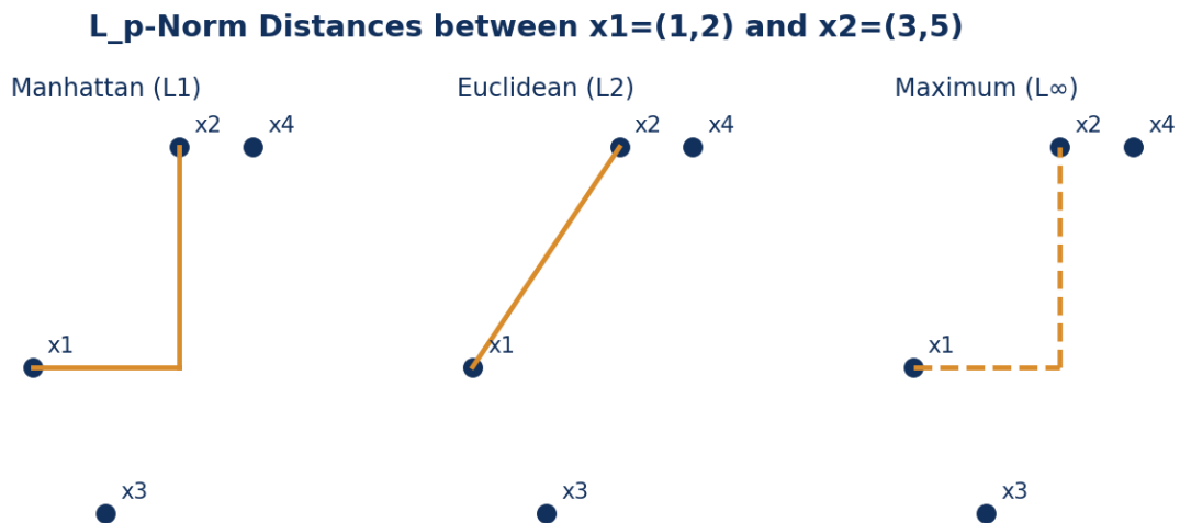
Figure: Manhattan (grid path), Euclidean (straight line), and Maximum (dashed grid) distance between x_1 and x_2 .
