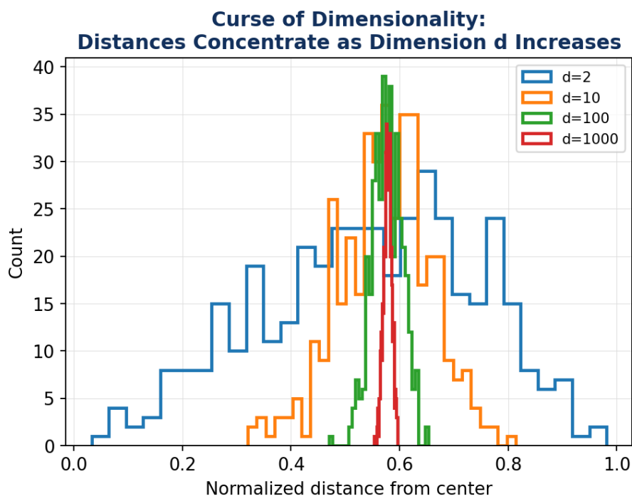
Figure: As dimensionality d grows, points' normalized distances from the center concentrate tightly — illustrating why 'almost all pairs are equidistant' in high dimensions.
