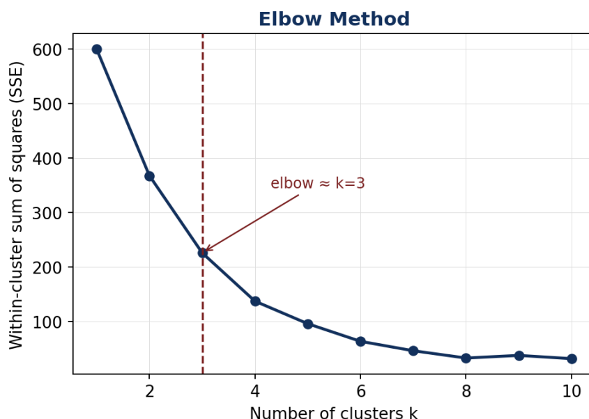
Figure: Elbow method — SSE drops sharply then flattens; the bend suggests the best k .
