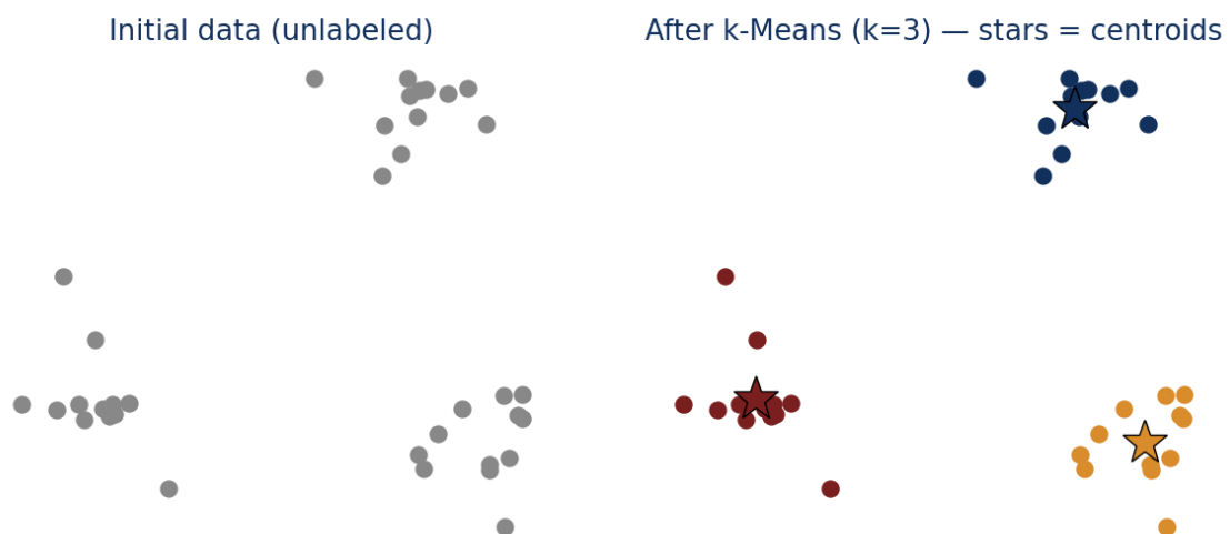
Figure: k-Means on unlabeled data (left) converges to k=3 clusters with centroids marked as stars (right).
