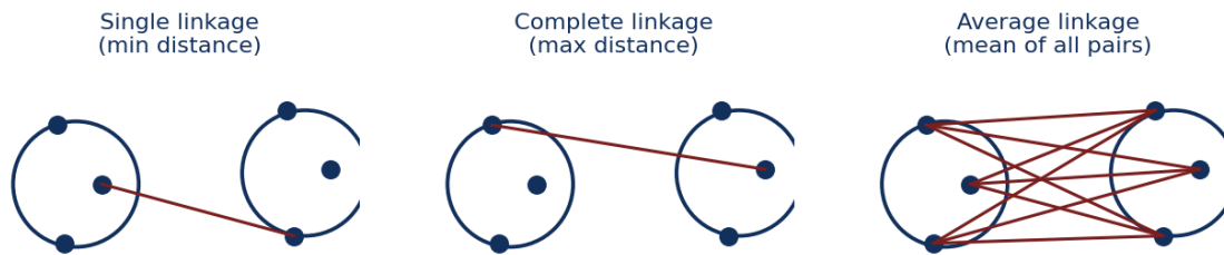
Figure: Single linkage uses the closest pair, complete linkage the farthest pair, average linkage the mean over all pairs between clusters G and H.
