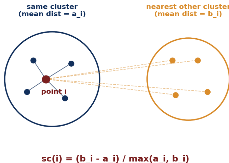
Figure: For point i , a_i is its mean distance to its own cluster; b_i is its mean distance to the nearest other cluster.
