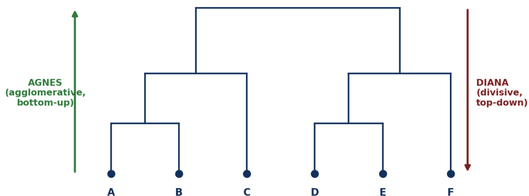
Figure: A dendrogram — AGNES merges bottom-up (green arrow), DIANA splits top-down (red arrow).
