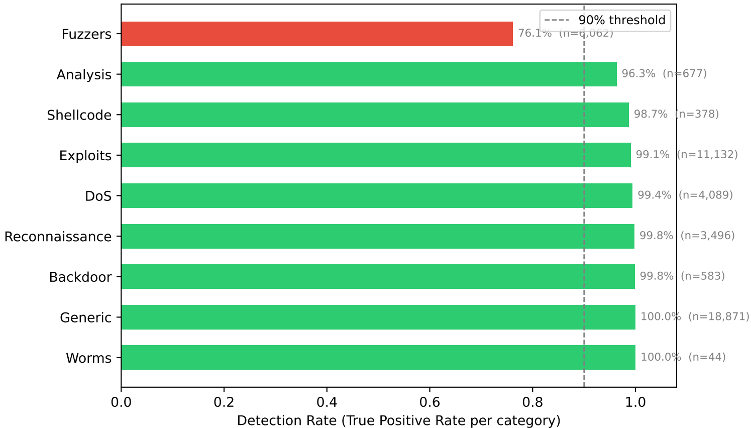
Per-Attack-Category Detection Rate (XGBoost)
