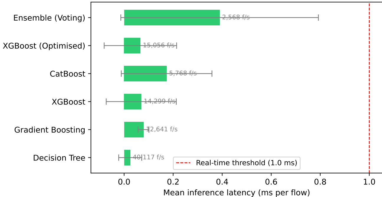
Per-Flow Inference Latency — Microgrid IDS Candidates
