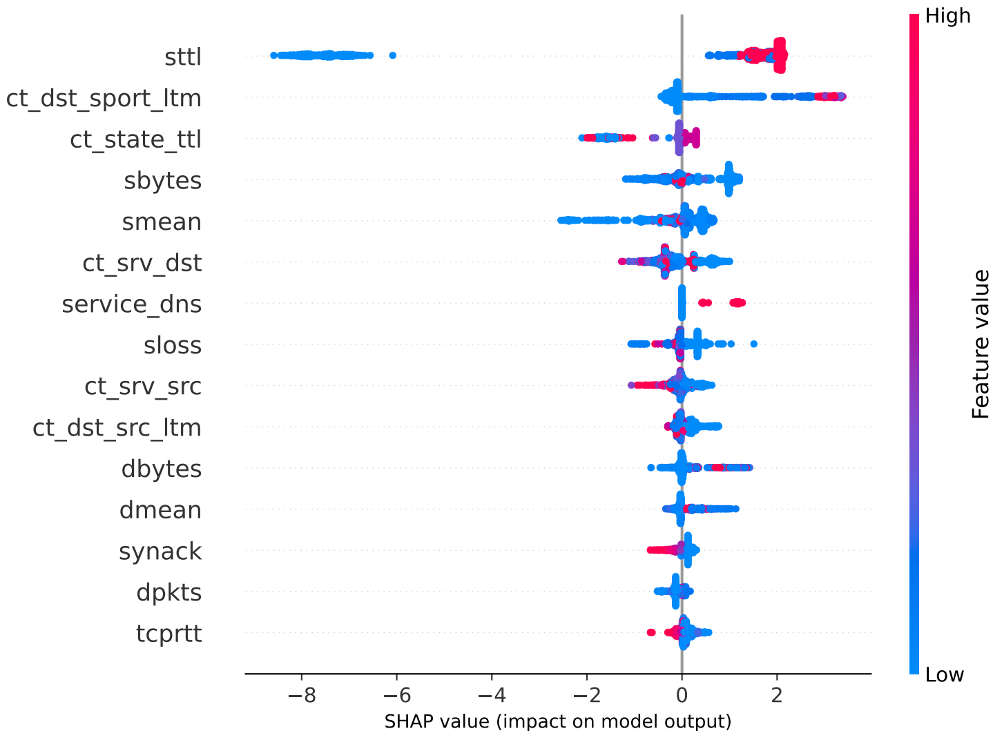
SHAP Feature Impact on Attack Detection (XGBoost)
