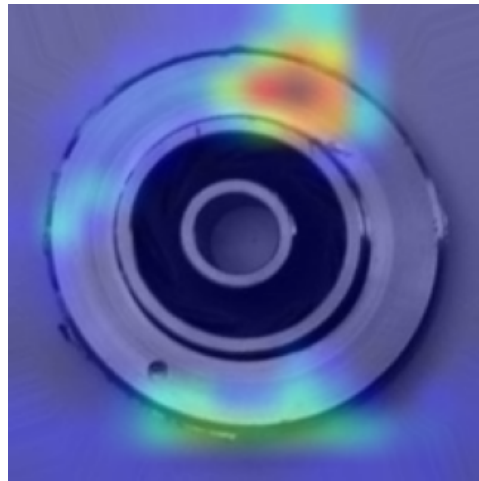
Custom CNN Pred: def_front Conf: 1.00
