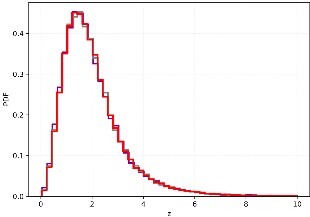
Redshift distribution
