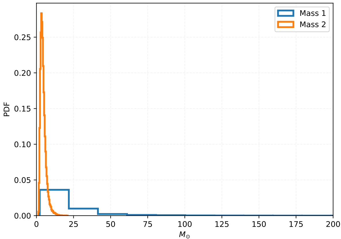
Mass distribution: NSBH
