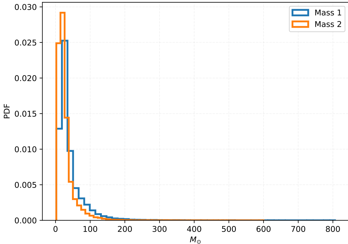
Mass distribution: stellar mass BHs (det frame)
