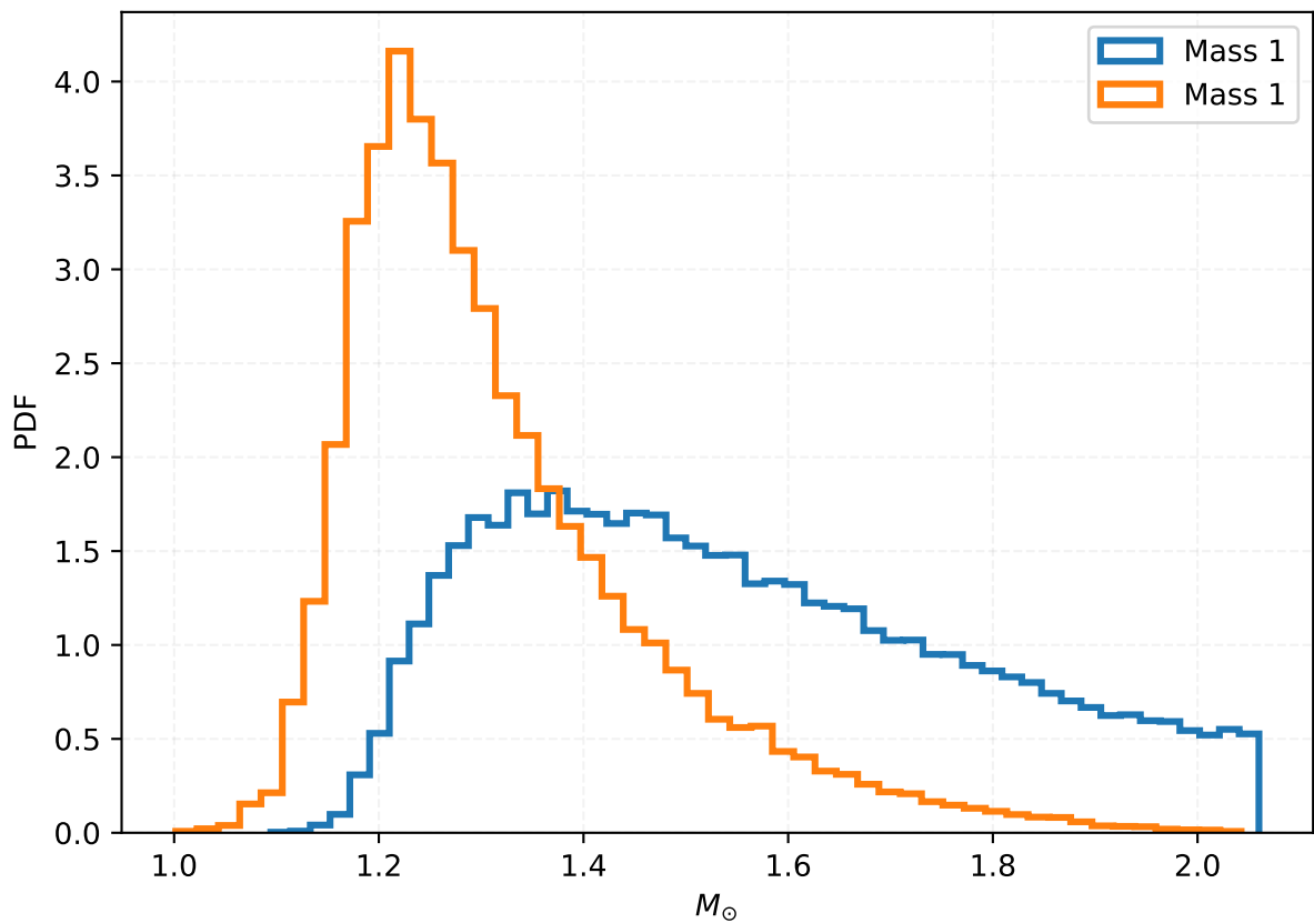
Mass distribution: BNS (source frame)
