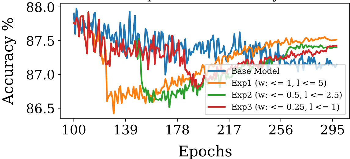
Top5 Valid Accuracy
