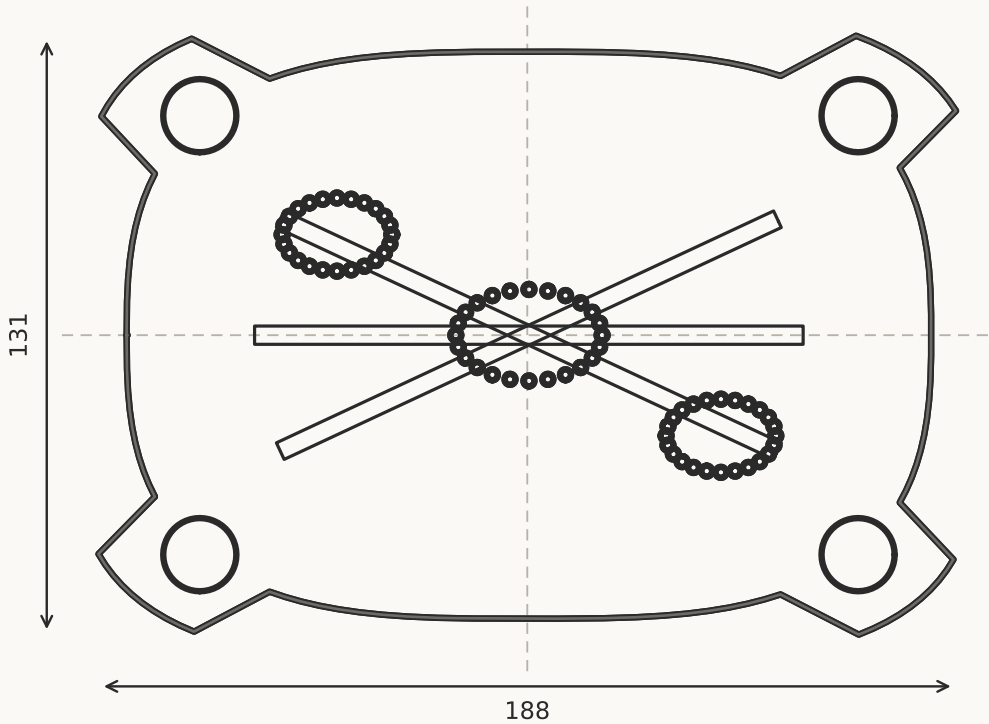
TOP VIEW
