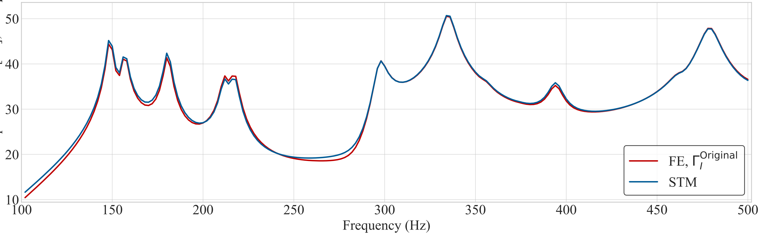
Comparison of FE variants and STM far-field sound power levels for "Simple elastic structure" RMSE: 0.54 dB
