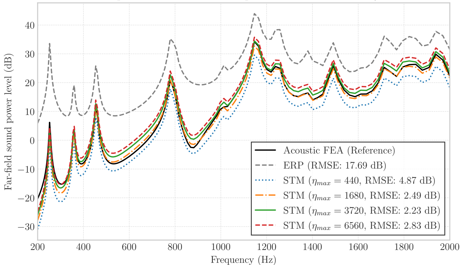
Comparison of far-field sound power levels for different \eta_{max}
