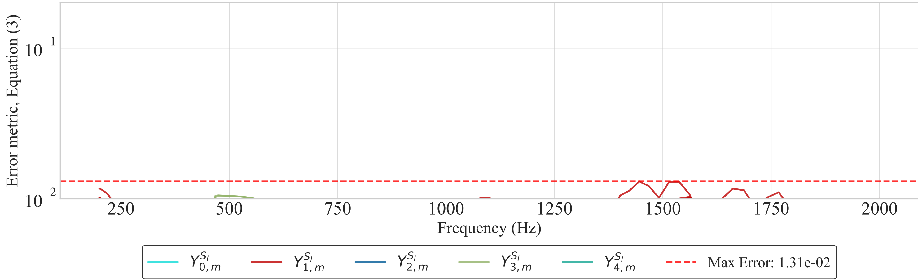
Error metric vs Frequency for individual interior pressure distributions, "Complex elastic structure"
