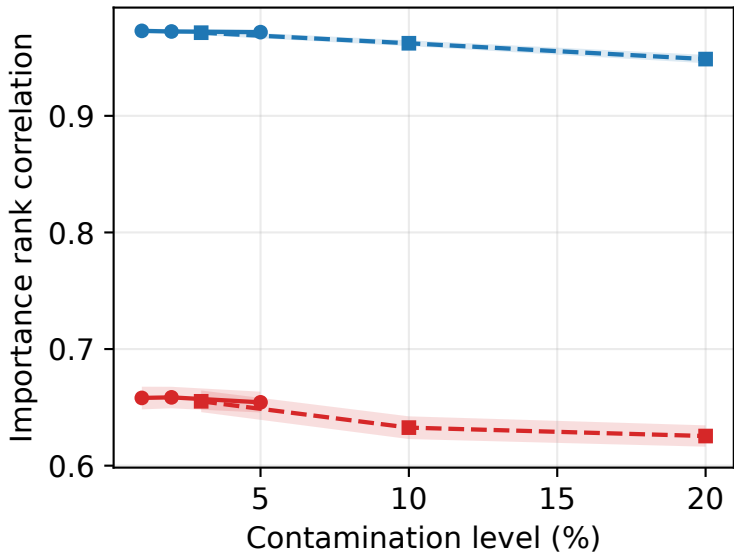
(a) Importance rank correlation
